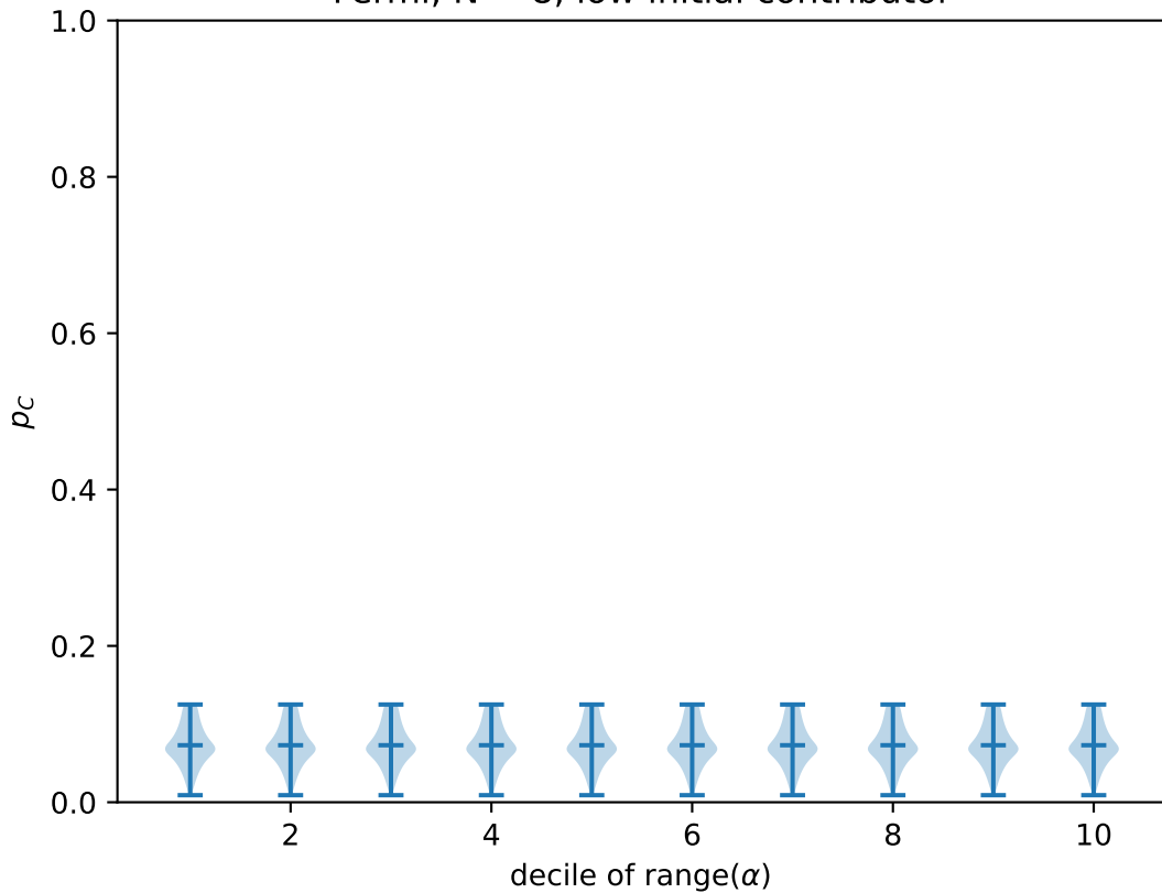
Fermi, N = 8 , low initial contributor
