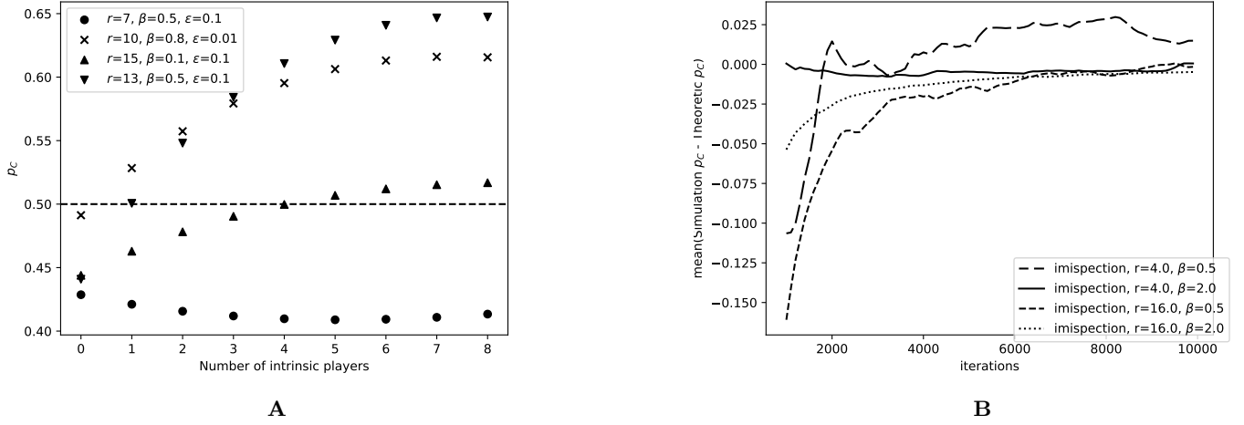
Figure 14: A : p_C in various parameter combinations at N = 8 , varying the number of players using an intrinsic population dynamic. B : for various parameter combinations, the mean value over numerous simulations of an 8 player population playing introspective imitation dynamics converging to the theoretic p_C .
