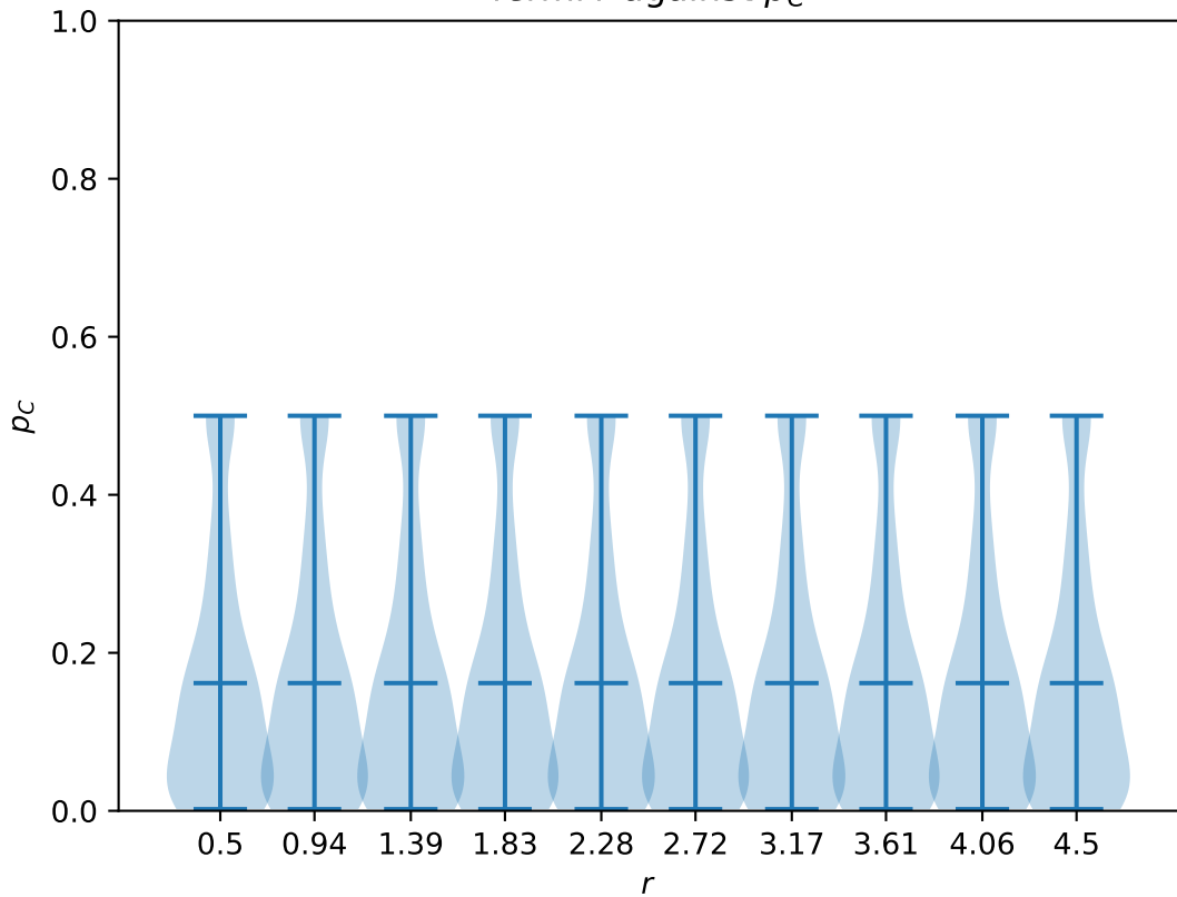
fermi r against p_c
