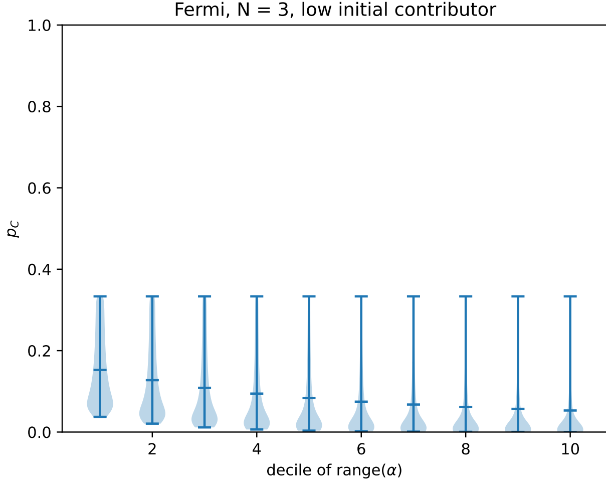
Figure 3: p_C under Fermi imitation dynamics as heterogeneity varies ( N = 3 , linear population, low mutant).
