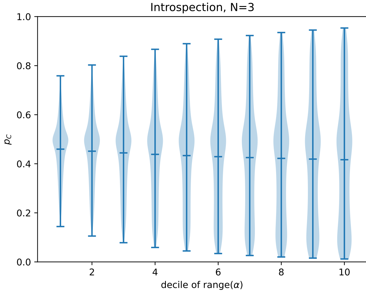
Figure 7: p_C under introspection dynamics ( N = 3 , linear population).
