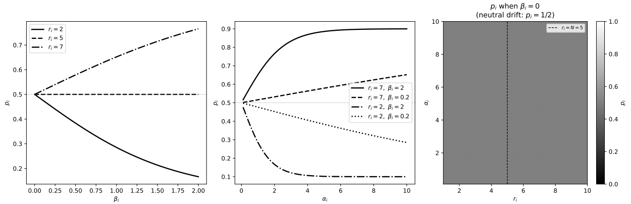
Figure 2: Structural properties of p_i for a single player with N = 5 , \mu_{i0} = \mu_{i1} = 0.1 . Left: p_i as a function of \beta_i ( \alpha_i = 2 ) for r_i < N , r_i = N , and r_i > N ; all curves pass through p_i = \frac{1}{2} at \beta_i = 0 (Remark 2). Centre: p_i as a function of \alpha_i for two values of r_i and \beta_i ; curves above (below) \frac{1}{2} correspond to r_i > N ( r_i < N ). Right: p_i(\alpha_i, r_i) at \beta_i = 0 , confirming p_i = \frac{1}{2} everywhere (Remark 2); the dashed line marks r_i = N .
