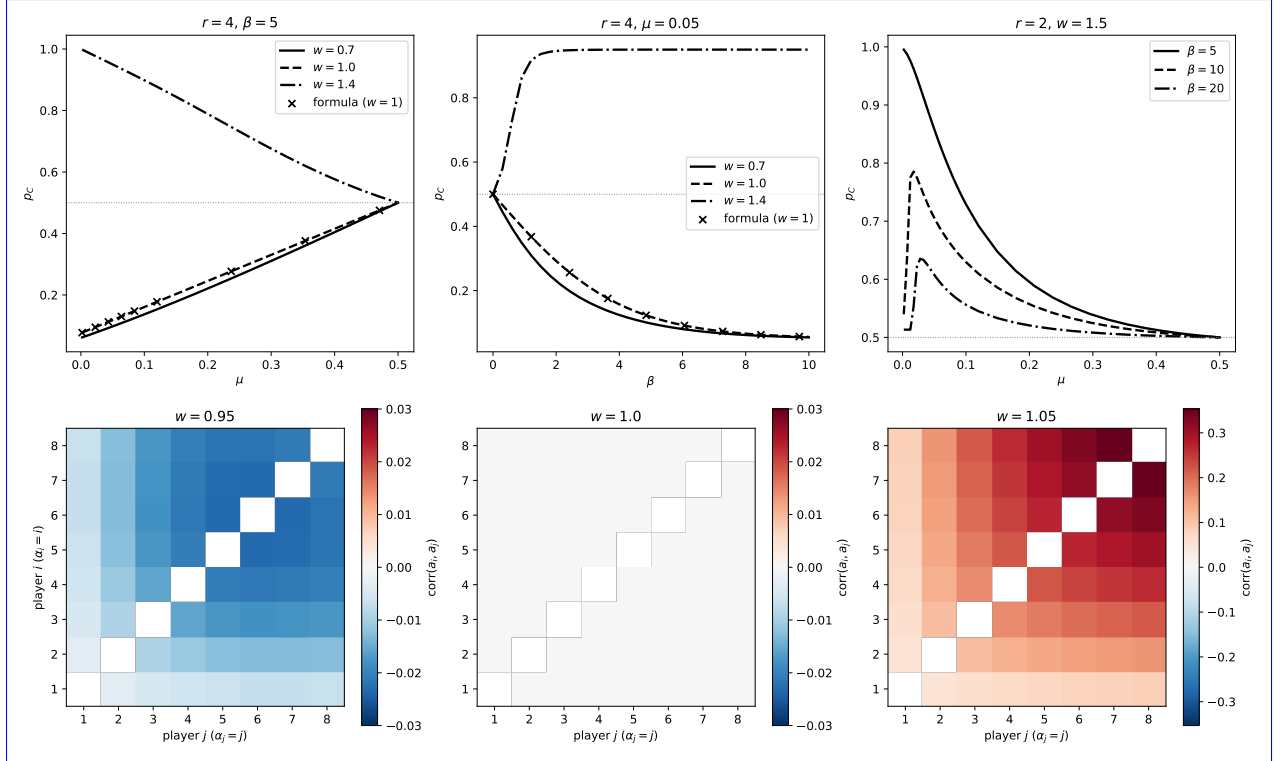
Figure 4: Mutation in the non-linear public goods game (15) with N = 8 ; the top row takes unit contributions ( \alpha_i = 1 ). All values were computed exactly from the full 2^N linear system using [5]. Top left: p_C as a function of the common symmetric mutation rate \mu at r = 4 , \beta = 5 , for discounting ( w = 0.7 ), the linear game ( w = 1 ), and synergy ( w = 1.4 ); the closed form of Corollary 2 matches the w = 1 values well. The w = 0.7 curve follows the additive pattern but is no longer affine, whilst the w = 1.4 curve starts near full cooperation and falls towards \frac{1}{2} . Top centre: p_C as a function of \beta at r = 4 , \mu = 0.05 . For w \leq 1 strong selection drives cooperation to the mutation floor \mu ; for w = 1.4 it selects the cooperative equilibrium and p_C approaches 1 - \mu . Top right: p_C as a function of \mu for a bistable synergy game ( r = 2 , w = 1.5 ). At \beta = 10 and \beta = 20 cooperation is maximised at a strictly positive mutation rate, which Proposition 4 rules out for additive games. Bottom row: pairwise correlations \text{corr}(a_i, a_j) under the stationary distribution for the heterogeneous group of Figure 1 (contributions \alpha_i = i , \beta = 0.5 ), at r = 4 and \mu = 0.05 . The axes give the player indices i and j , which, since \alpha_i = i , also order the players by contribution; diagonals are omitted and the colour scales differ between panels. For w = 1 every entry is zero (Theorem 1); for w = 0.95 all pairs are weakly negatively correlated; for w = 1.05 the correlations are positive and increase with both players' contributions.
