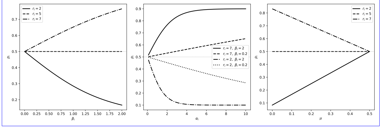
Figure 2: Structural properties of p_i for a single player with N = 5 and, unless varied, symmetric mutation \mu_{iC} = \mu_{iD} = 0.1 . Left: p_i as a function of \beta_i ( \alpha_i = 2 ) for r_i < N , r_i = N , and r_i > N ; all curves pass through p_i = \frac{1}{2} at \beta_i = 0 (Remark 2). Centre: p_i as a function of \alpha_i for two values of r_i and \beta_i ; curves above (below) \frac{1}{2} correspond to r_i > N ( r_i < N ). Right: p_i as a function of the symmetric mutation rate \mu_{iC} = \mu_{iD} = \mu ( \alpha_i = 2 , \beta_i = 2 ) for r_i < N , r_i = N , and r_i > N ; each line is affine in \mu (Proposition 4) and reaches p_i = \frac{1}{2} at \mu = \frac{1}{2} .
