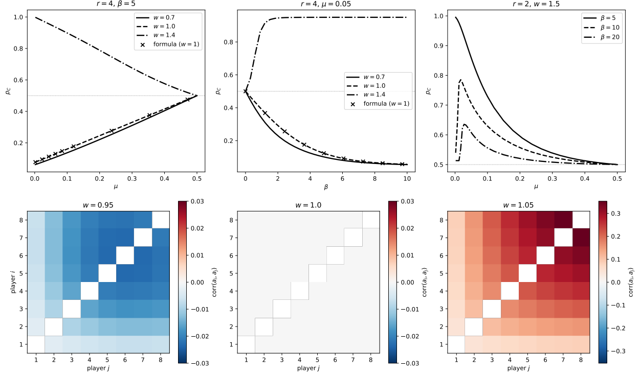
Figure 4: Mutation in the non-linear public goods game (13) with N = 8 and \alpha = 1 . All values were computed exactly from the full 2^N linear system using [5]. Top left: p_C as a function of the common symmetric mutation rate \mu at r = 4, \beta = 5 , for discounting ( w = 0.7 ), the linear game ( w = 1 ), and synergy ( w = 1.4 ); the closed form of Corollary 2 matches the w = 1 values well. The w = 0.7 curve follows the additive pattern but is no longer affine, whilst the w = 1.4 curve starts near full cooperation and falls towards \frac{1}{2} . Top centre: p_C as a function of \beta at r = 4, \mu = 0.05 . For w \leq 1 strong selection drives cooperation to the mutation floor \mu ; for w = 1.4 it selects the cooperative equilibrium and p_C approaches 1 - \mu . Top right: p_C as a function of \mu for a bistable synergy game ( r = 2, w = 1.5 ). At \beta = 10 and \beta = 20 cooperation is maximised at a strictly positive mutation rate, which Proposition 2 rules out for additive games. Bottom row: pairwise correlations \text{corr}(a_i, a_j) under the stationary distribution for the heterogeneous group of Figure 1 (contributions \alpha_i = i, \beta = 0.5 ), at r = 4 and \mu = 0.05 ; diagonals are omitted and the colour scales differ between panels. For w = 1 every entry is zero (Theorem 1); for w = 0.95 all pairs are weakly negatively correlated; for w = 1.05 the correlations are positive and increase with both players' contributions.
