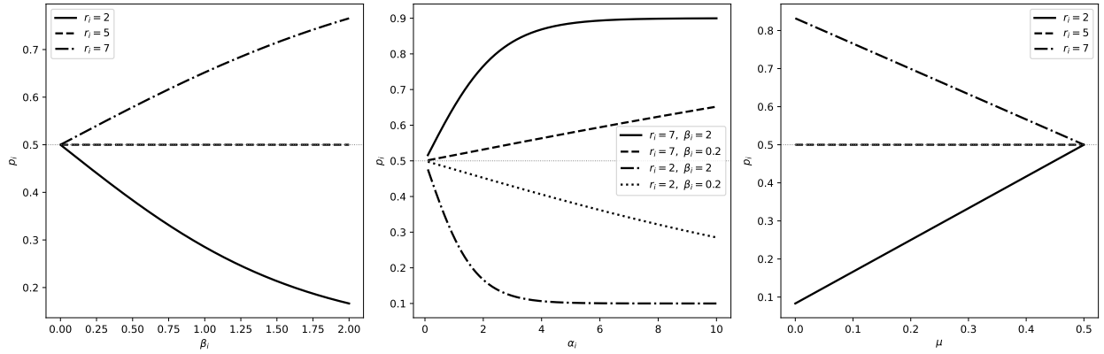
Figure 2: Structural properties of p_i for a single player with N = 5 and, unless varied, symmetric mutation \mu_{i0} = \mu_{i1} = 0.1 . Left : p_i as a function of \beta_i ( \alpha_i = 2 ) for r_i < N , r_i = N , and r_i > N ; all curves pass through p_i = \frac{1}{2} at \beta_i = 0 (Remark 2). Centre : p_i as a function of \alpha_i for two values of r_i and \beta_i ; curves above (below) \frac{1}{2} correspond to r_i > N ( r_i < N ). Right : p_i as a function of the symmetric mutation rate \mu_{i0} = \mu_{i1} = \mu ( \alpha_i = 2 , \beta_i = 2 ) for r_i < N , r_i = N , and r_i > N ; each line is affine in \mu (Proposition 2) and reaches p_i = \frac{1}{2} at \mu = \frac{1}{2} .
