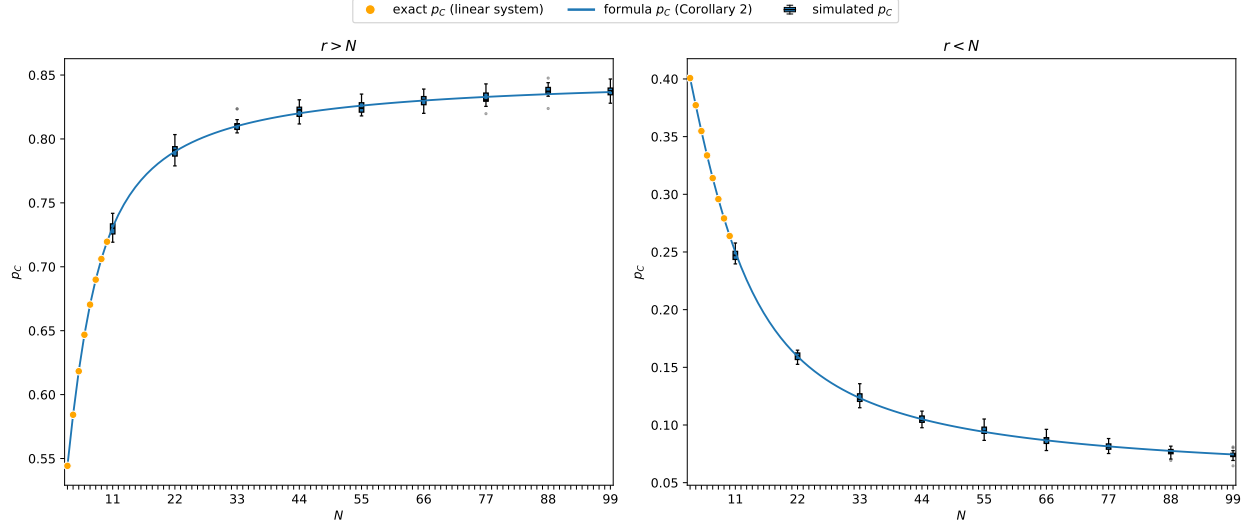
Figure 1: Validation of formula (12) on a heterogeneous group with \alpha_i = i , \beta = 0.5 , \mu_{i0} = 0.05 , \mu_{i1} = 0.15 . Left : r = 2N (so r > N for all N ). Right : r = N/2 (so r < N for all N ). Orange dots: exact p_C from the full 2^N linear system (feasible only for small N ). Blue curve: formula (12) (Corollary 2). Blue boxes: distribution of p_C across 19 independent runs of 5,000 simulation steps each (with the first 500 steps discarded as warm-up; outliers shown). All values were obtained using [3].
