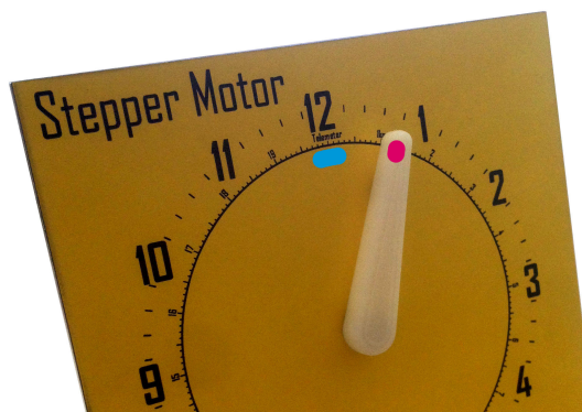
Figure 11 - Position of the Reed-Relay and the magnet .
