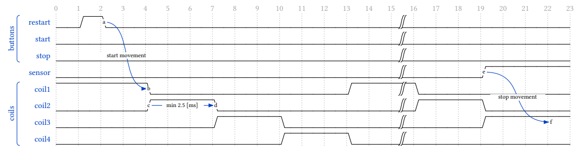
Figure 5 - Chrono Scenario - Restart
