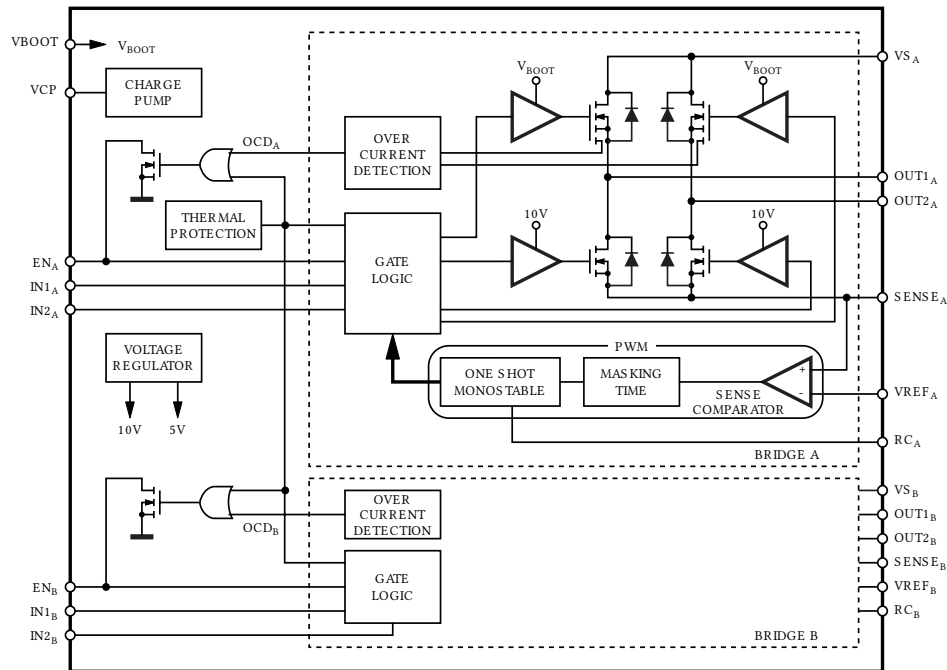
Figure 8 - Block diagram of the L6207N H-bridge circuit [4]
