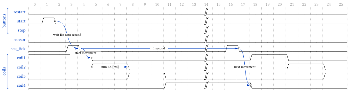
Figure 6 - Chrono Scenario - Start
