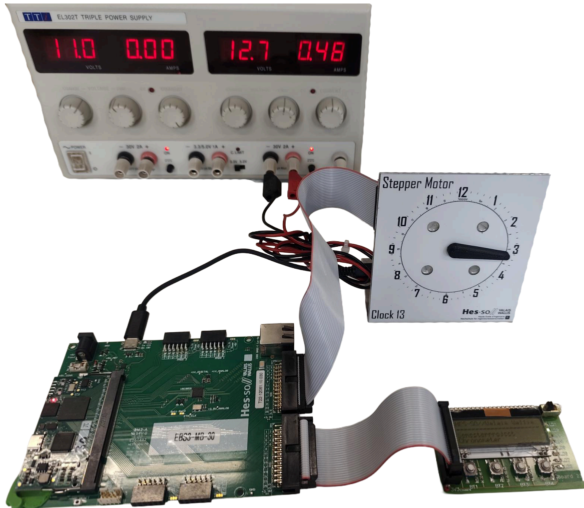
Figure 1 - Hardware setup Chrono (EBS3)
