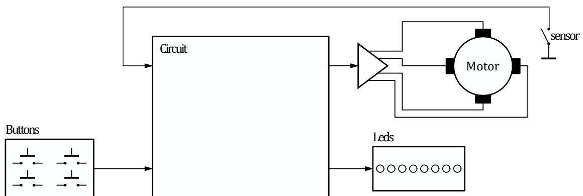
Figure 3 - Circuit of the chrono
