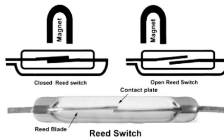
Figure 10 - Reed relais [6]
