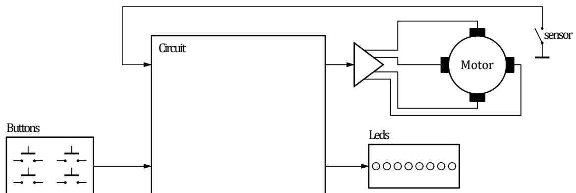
Figure 3 - Circuit du chrono
