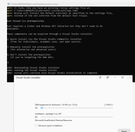
Figure 2 - MSVC installation through rustup
