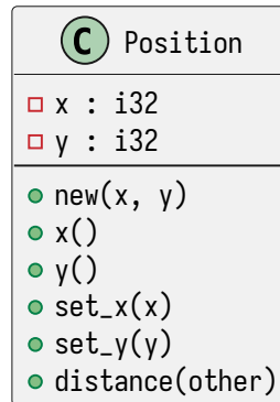
Figure 1 - The Position struct represents a point in 2D space with x and y coordinates.
