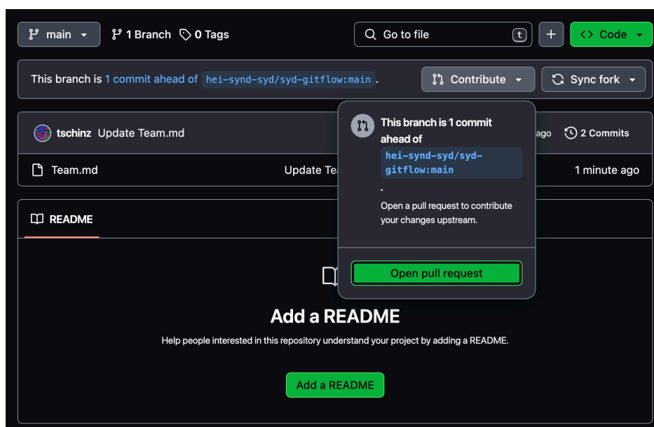
Figure 33 - Create Pull Request on Github
