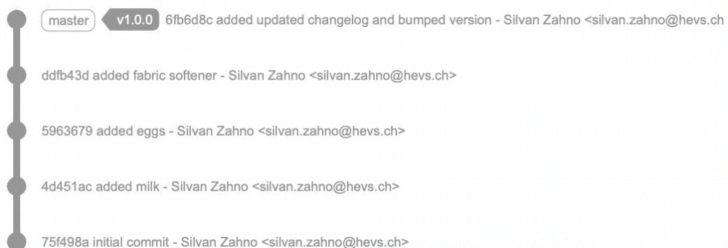
Figure 17 - Five commits on the local repo, each commit has its own identification
