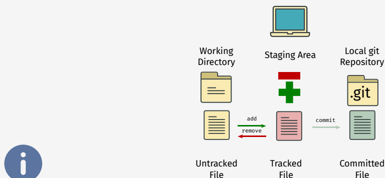
Figure 16 - Types of local Git operations
