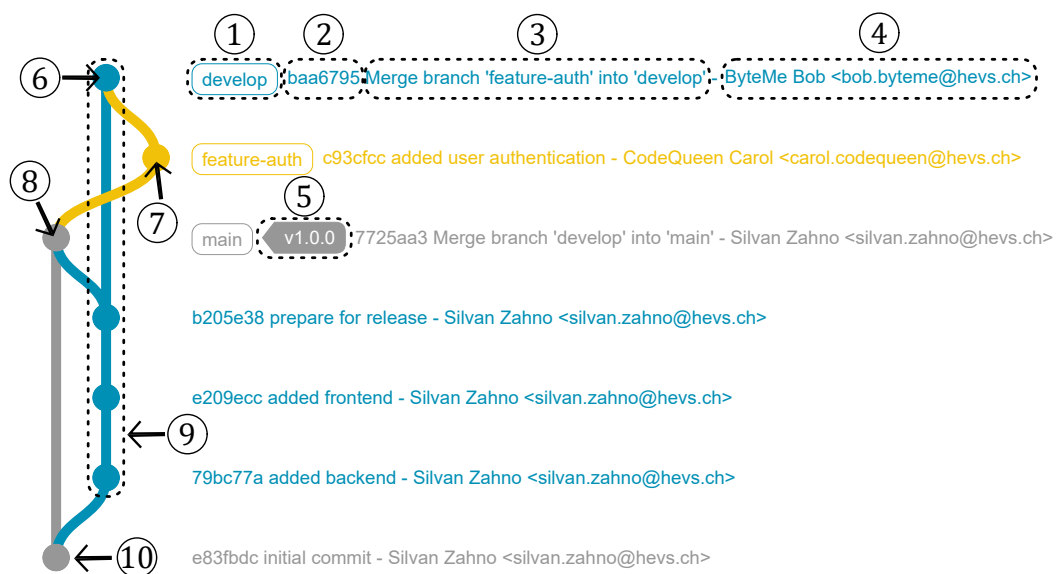
Figure 31 - Example of a Gitgraph
