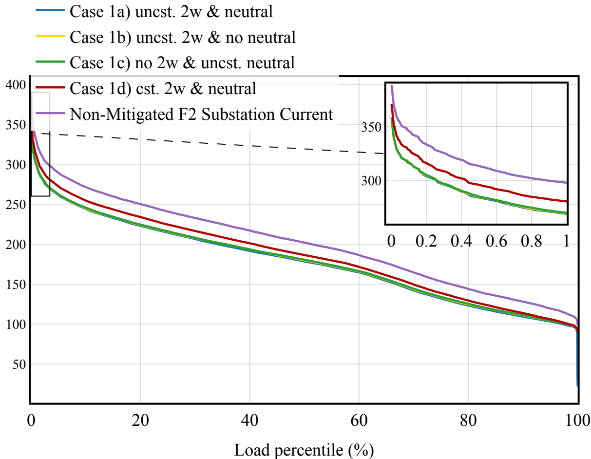
Maximum Feeder F2 Substation Phase Current (A)
