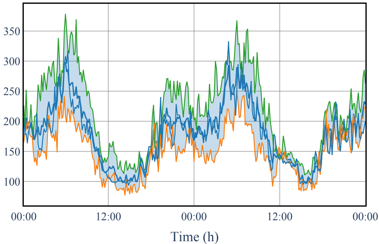
Feeder F2 Substation Current (A) Before Unbalance Mitigation
