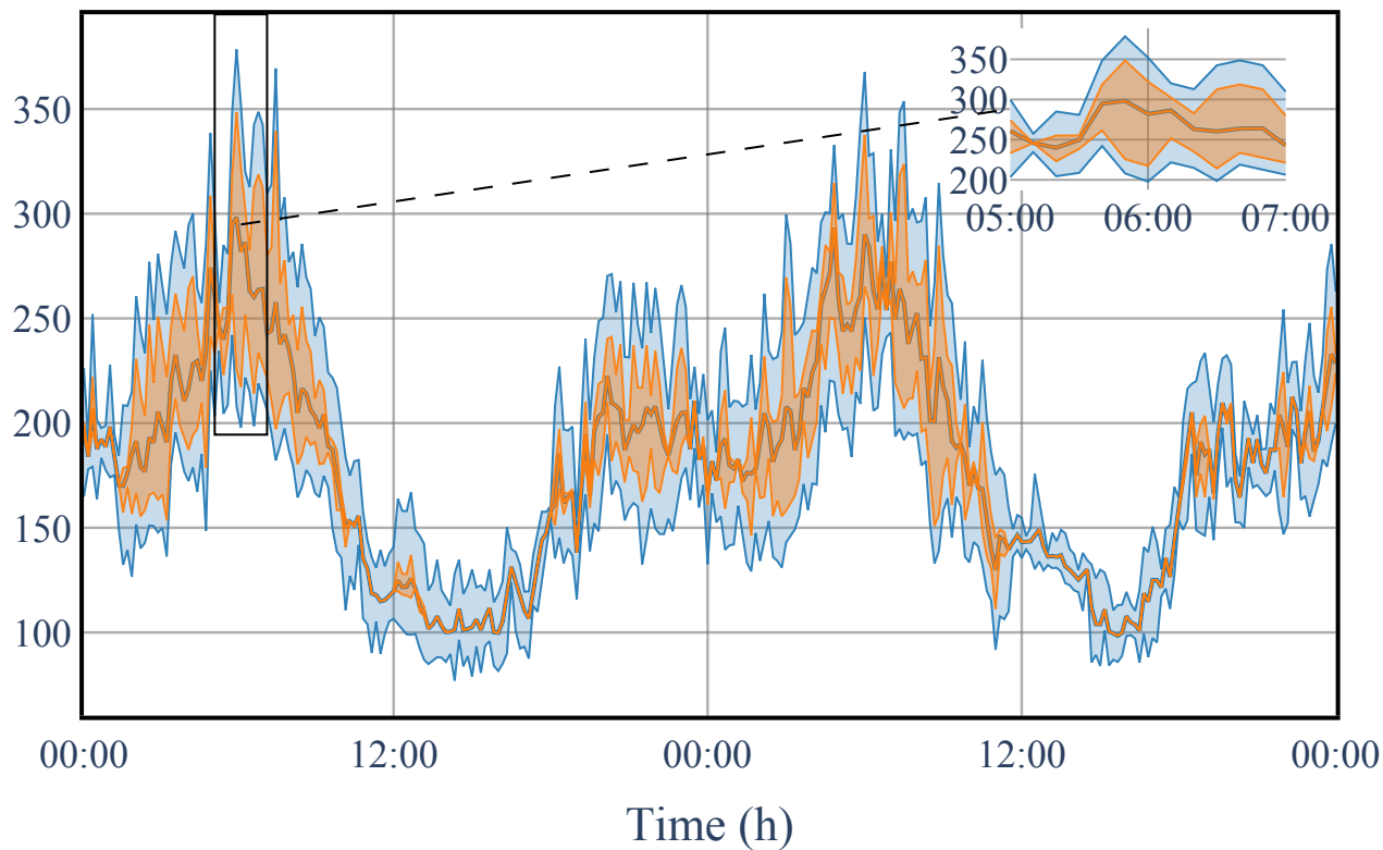
Feeder F2 Substation Current (A)
