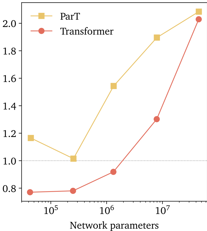
Training time gain (AMP)
