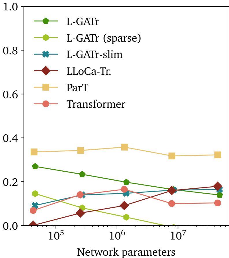
Training memory reduction (compile)
