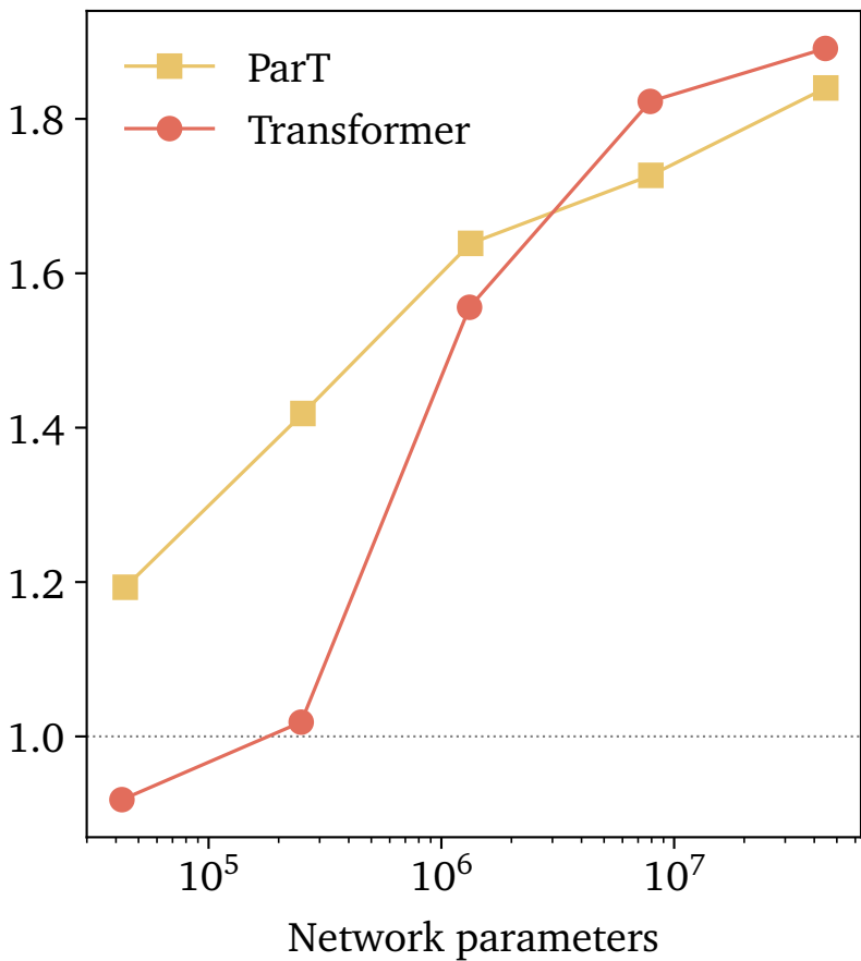
GPU inference time gain (AMP)
