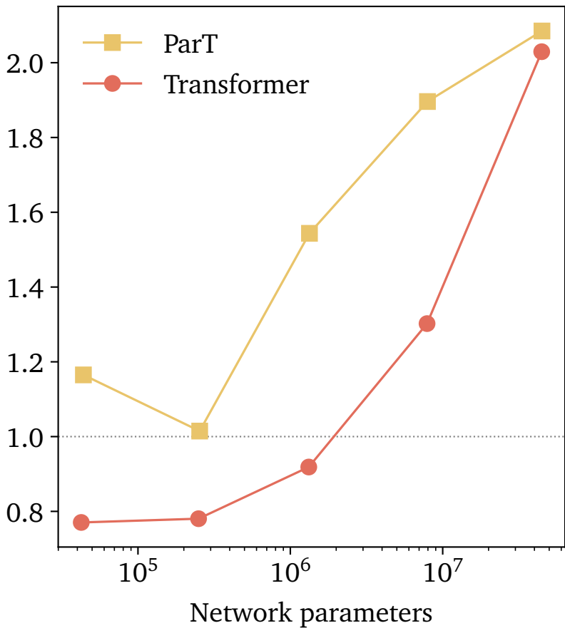
GPU training time gain (AMP)
