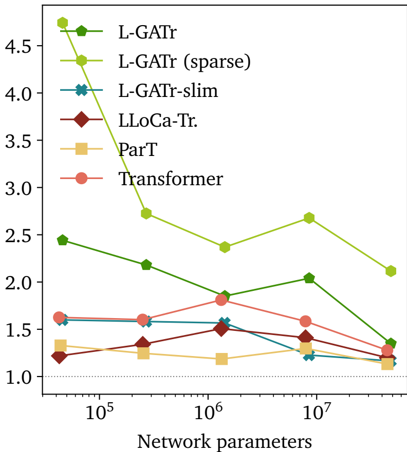
CPU inference time gain (compile)
