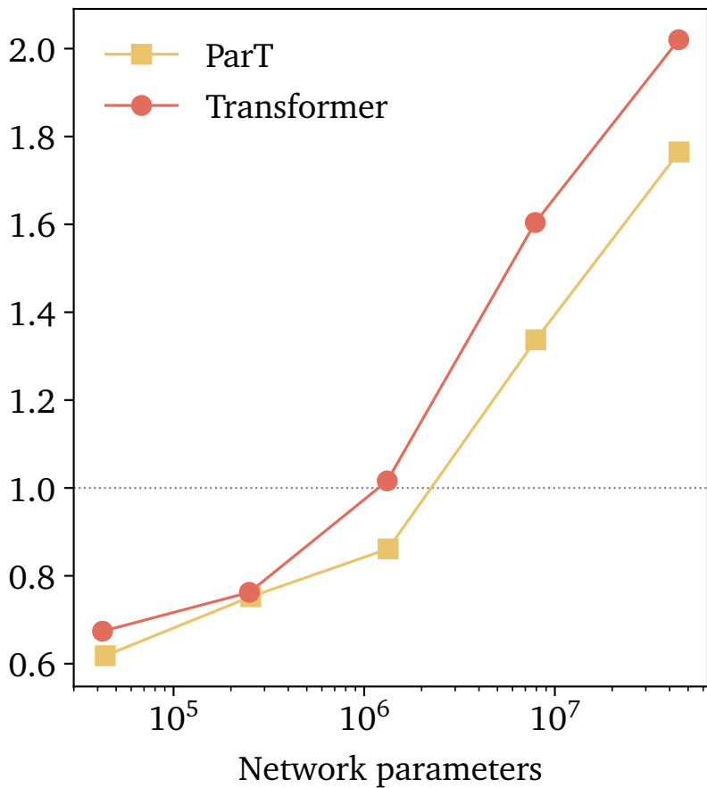
CPU inference time gain (AMP)
