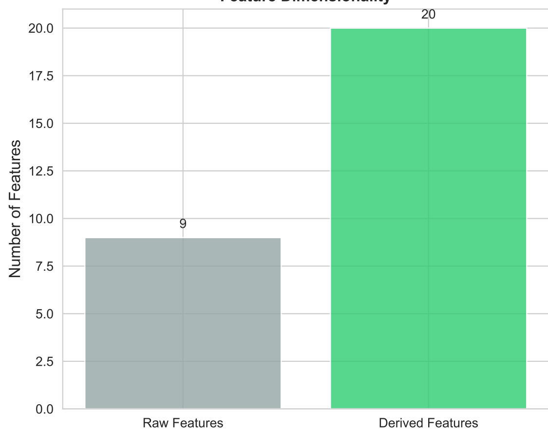
Feature Dimensionality
