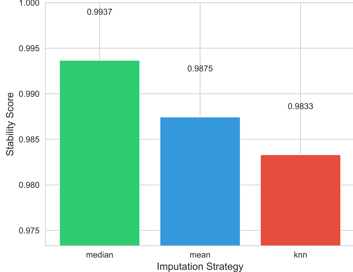
RQ1: Prediction Stability by Imputation Strategy
