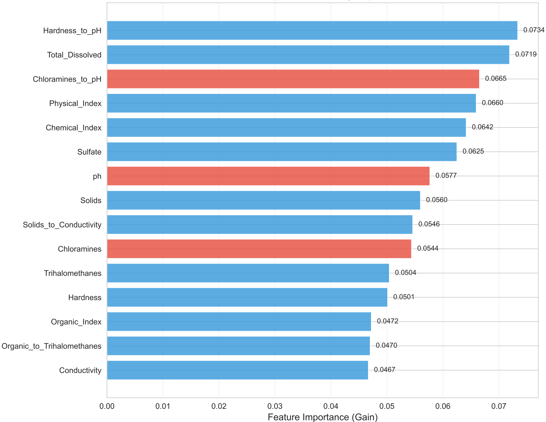
RQ5: Top 15 Features by Importance
