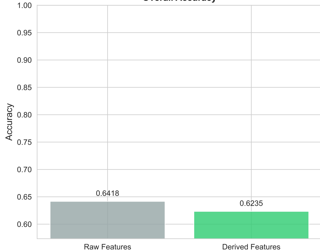
Overall Accuracy
