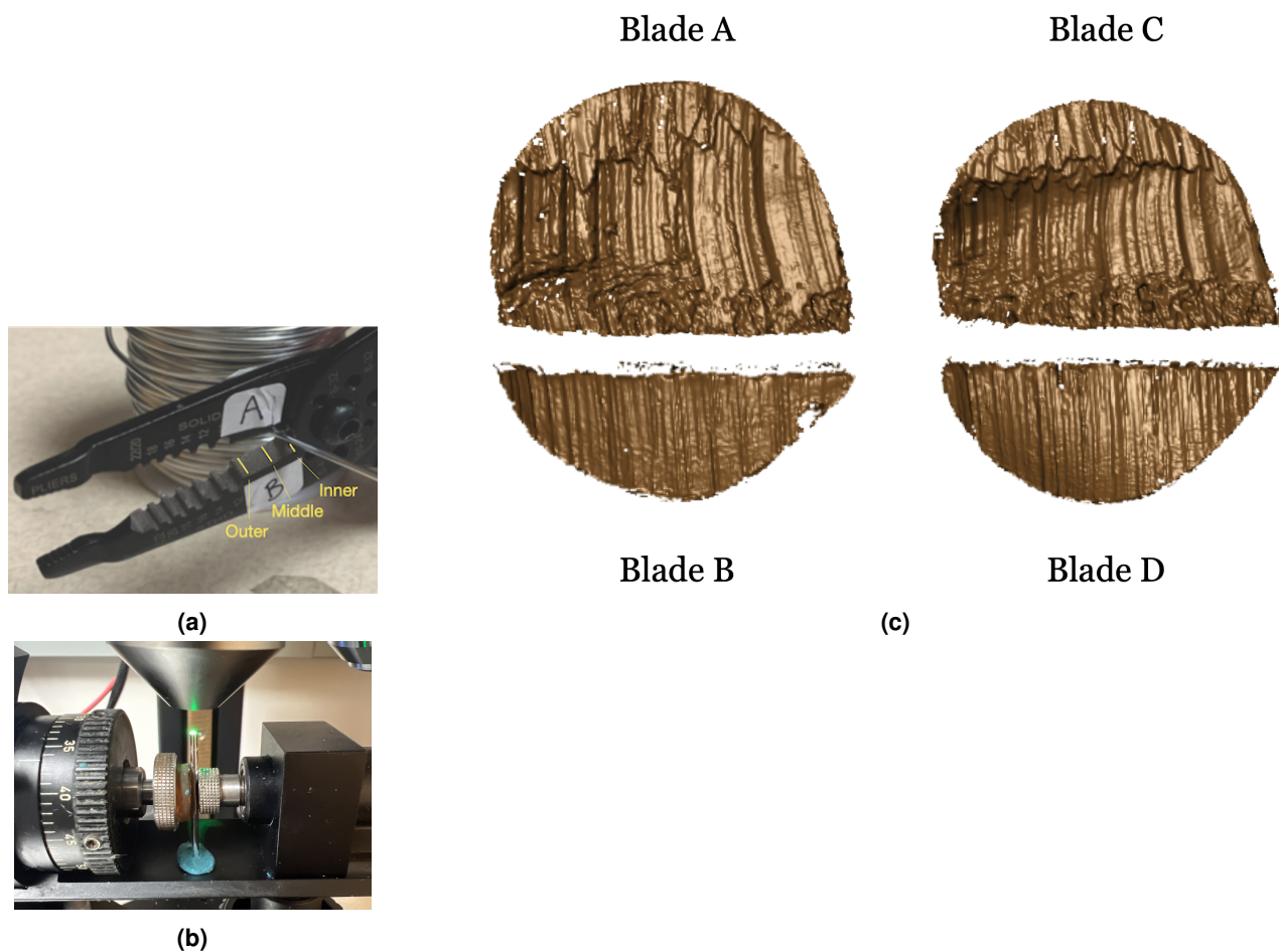
Figure 2. (a) A Kaiweets KWS-105 wire cutter with inner, middle, and outer locations marked. (b) A confocal microscope used to scan wire-cut surfaces. (c) Four samples obtained from blades A, B, C, and D after separating the cut edges. Figure width and height are tuned manually. For full figure requirements, see https://www.nature.com/sdata/publish/submission-guidelines#figures .
