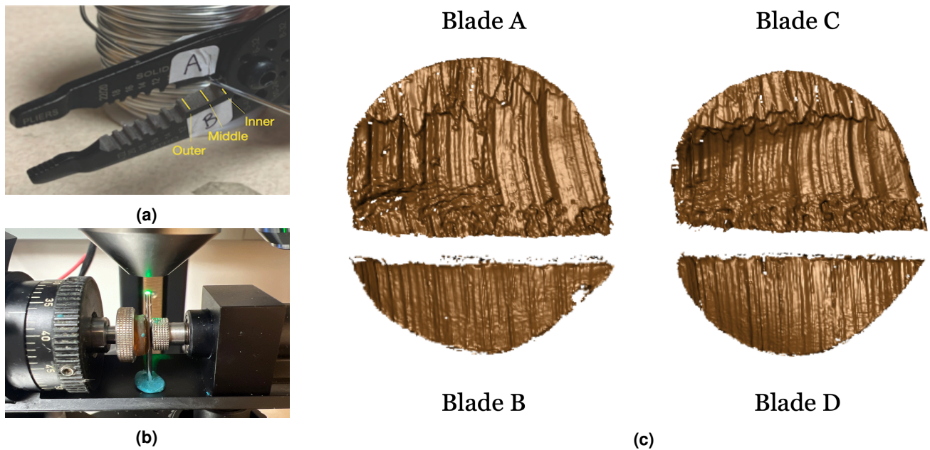
Figure 2. (a) A Kaiweets wire cutter of model KWS-105 was used to cut the wire, with inner, middle, and outer locations marked. (b) A confocal microscope was used to scan the wire-cut surfaces. (c) After separating edges by the connecting position, we obtained 4 samples - 2 samples from blade A and B, and others from blade C and D. width and height are tuned manually | full requirements see https://www.nature.com/sdata/publish/submission-guidelines#figures
