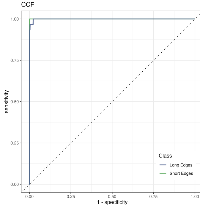
Figure 9. ROC curves for CCF-based classification. Curves compare same-source pairs with different-tool pairs separately for long and short edge classes; same-tool different-source pairs are excluded. The dotted diagonal indicates chance-level classification.
