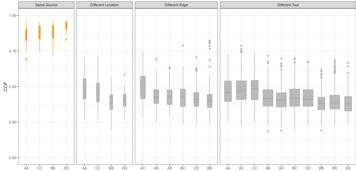
Figure 8. CCF distributions across comparison classes. Facets are ordered from left to right by decreasing expected similarity: same source, different location, different edge, and different tool. Orange boxplots show same-source comparisons; gray boxplots show different-source comparisons. Horizontal-axis labels identify the paired edges.
