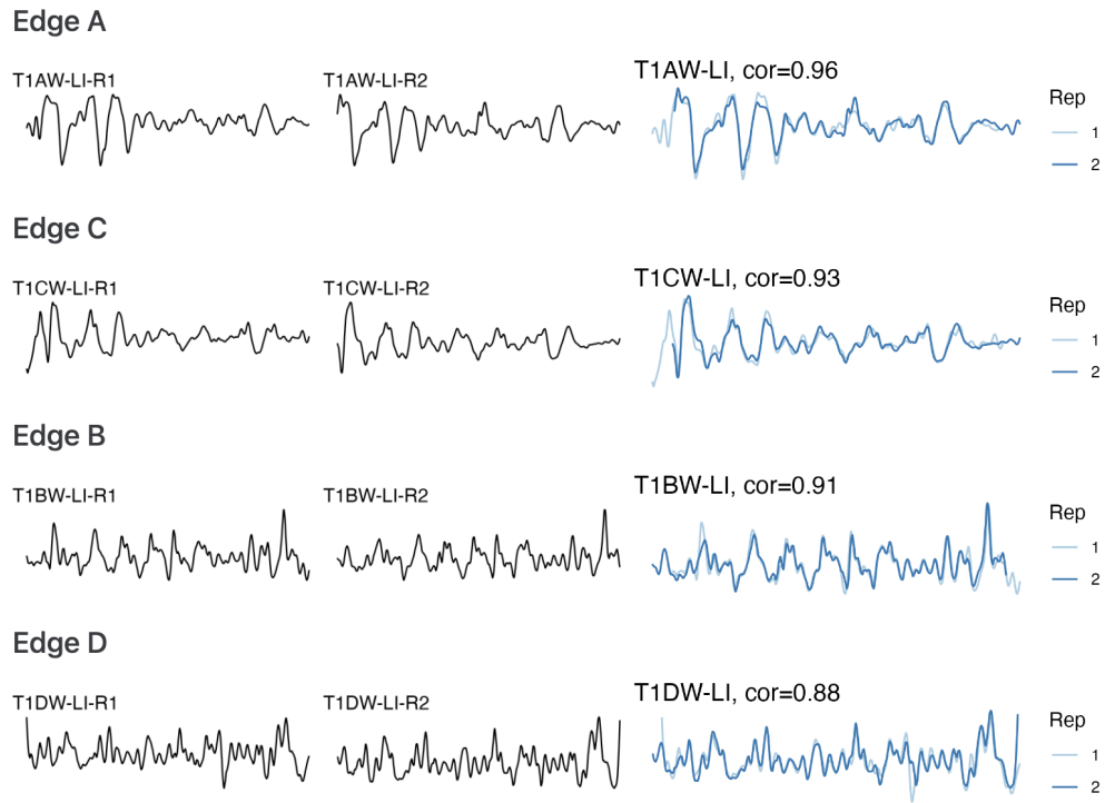
Figure 5. Same-source signal alignment. Rows correspond to cut surfaces A, C, B, and D. The first two columns show signals extracted from the replicate scans in Figure 4; the third column overlays the aligned signals and reports their CCF values.
