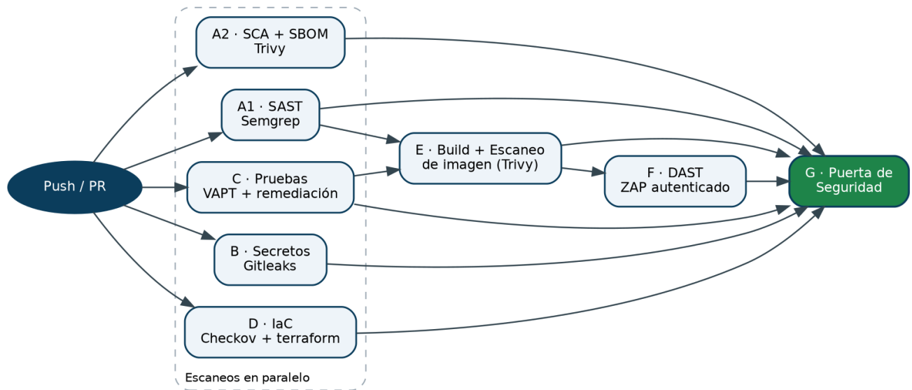
FleetSec — Pipeline DevSecOps (fan-out / fan-in, &lt;=15 min)
