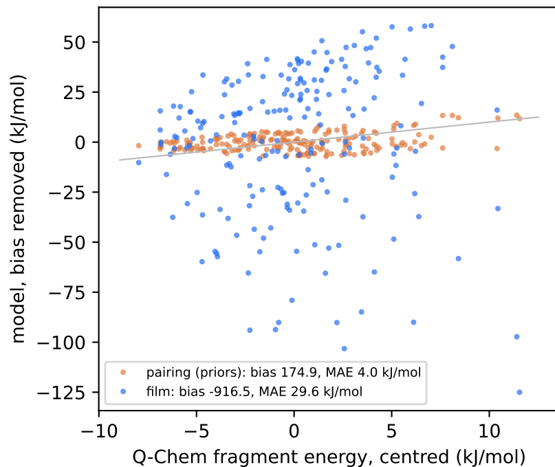
H3O+ monomers (200 frames)
