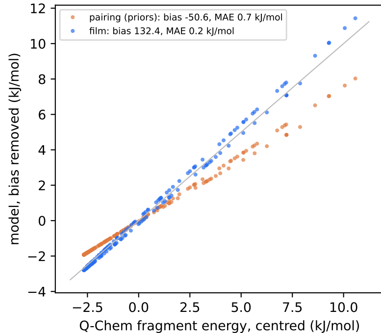
OH- monomers (200 frames)
