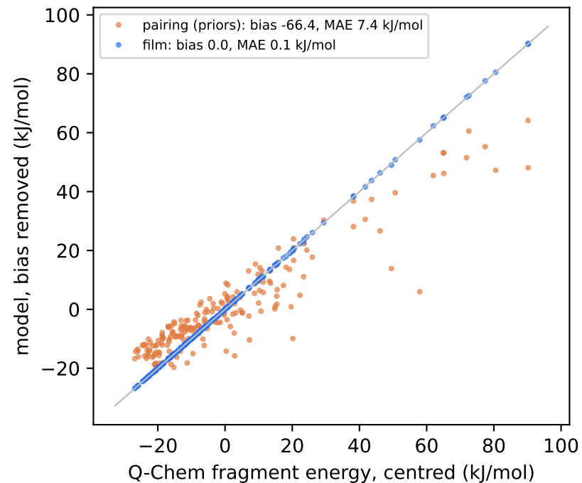
H2O monomers (200 frames)
