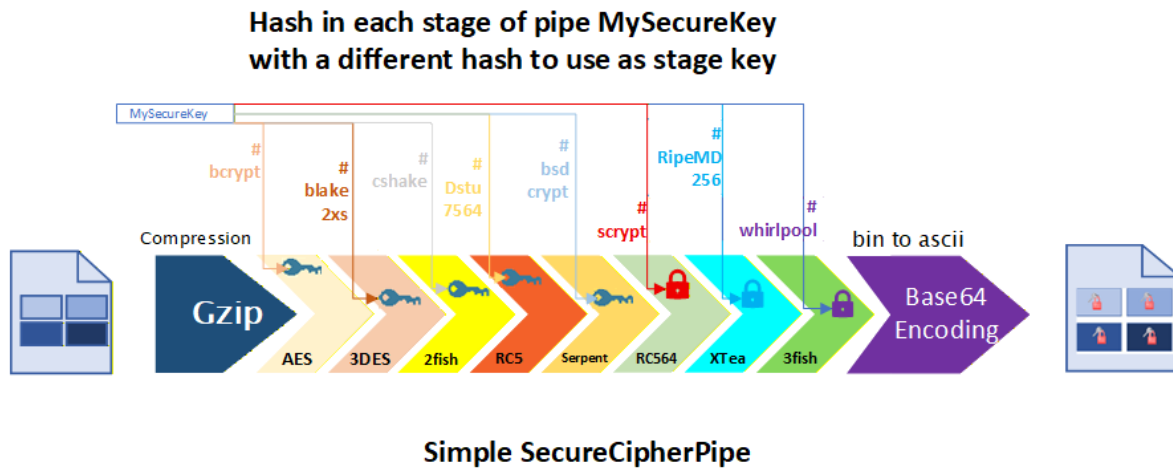
Figure 5: Simple SecureCipherPipe
