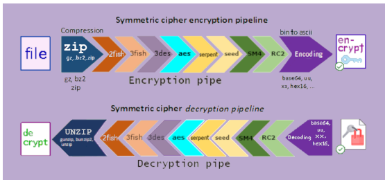
Figure 1: Cipher Pipeline
