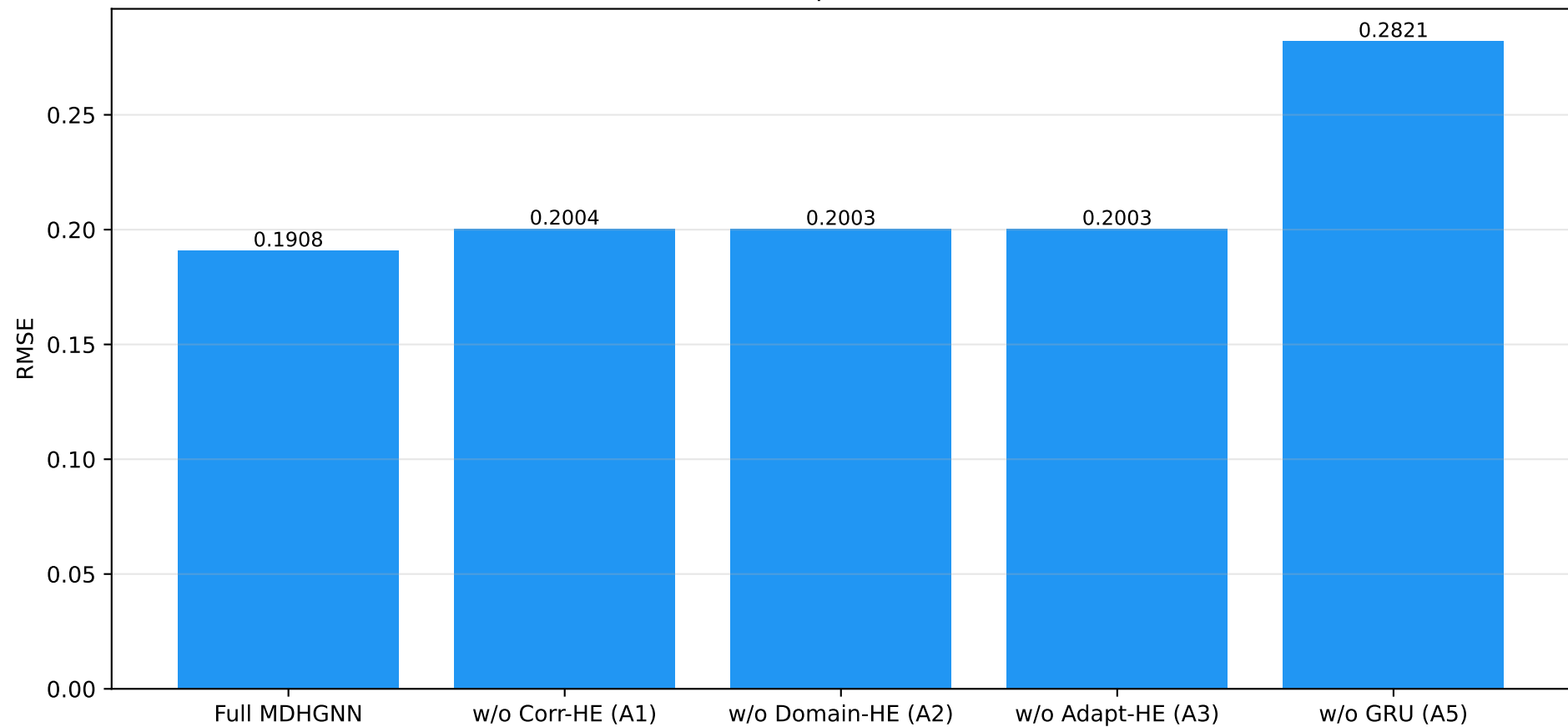
Model Comparison - RMSE
