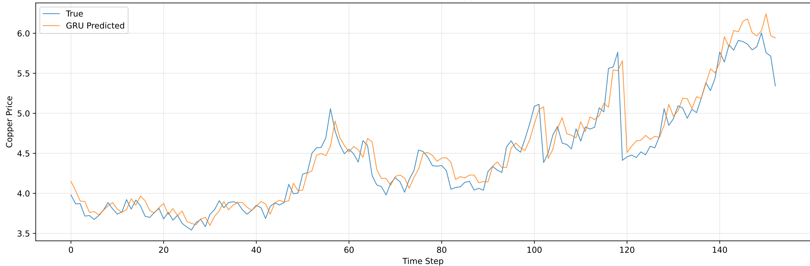
GRU - True vs Predicted Copper Price
