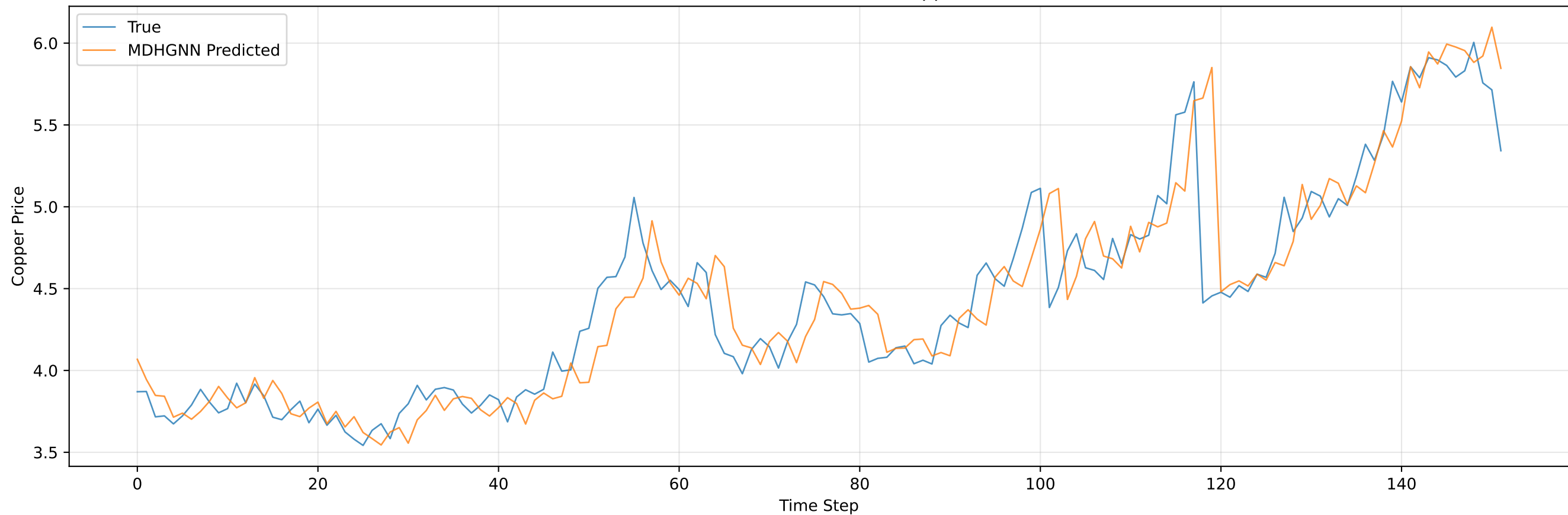
MDHGNN - True vs Predicted Copper Price
