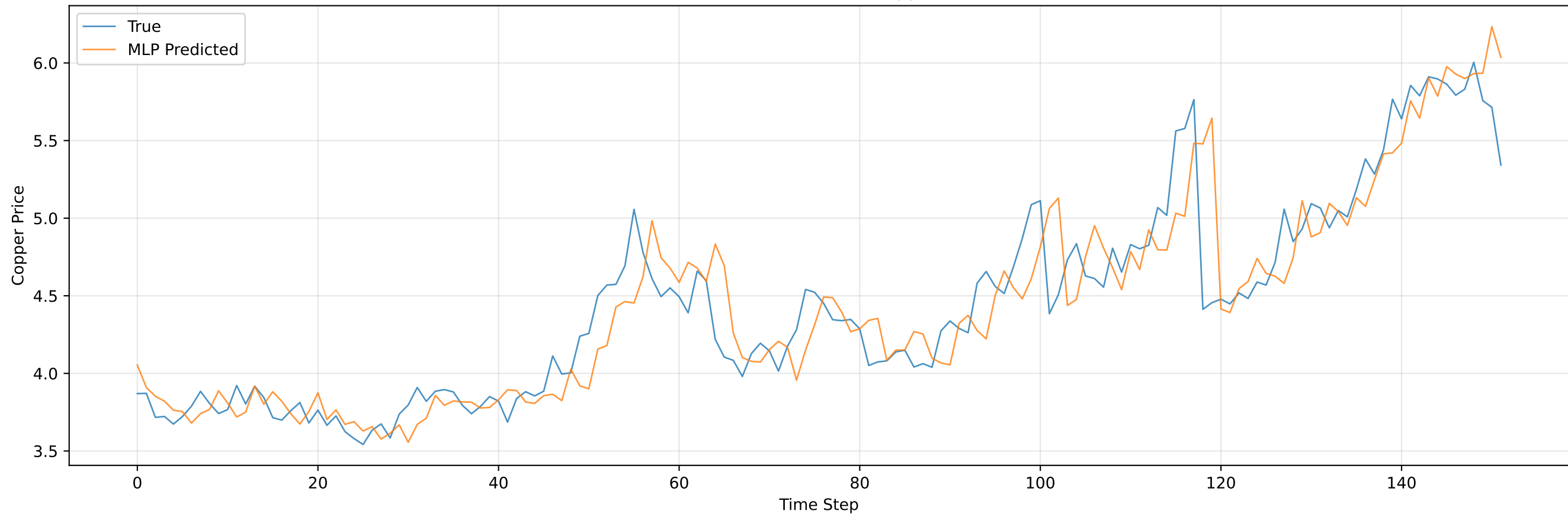
MLP - True vs Predicted Copper Price
