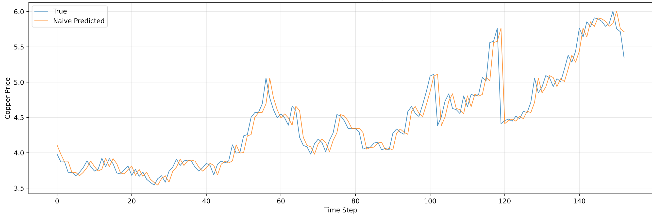
Naive - True vs Predicted Copper Price
