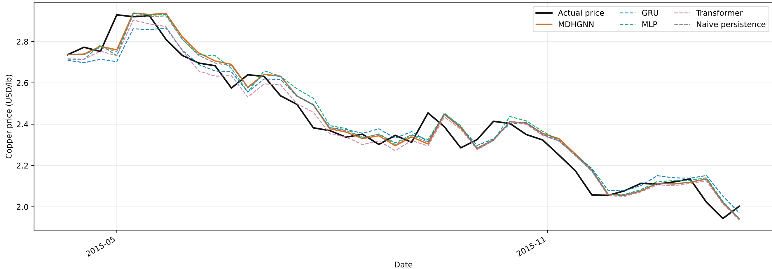
Test-set copper price predictions, h=1 Test period: 2015-04-10 to 2016-01-22
