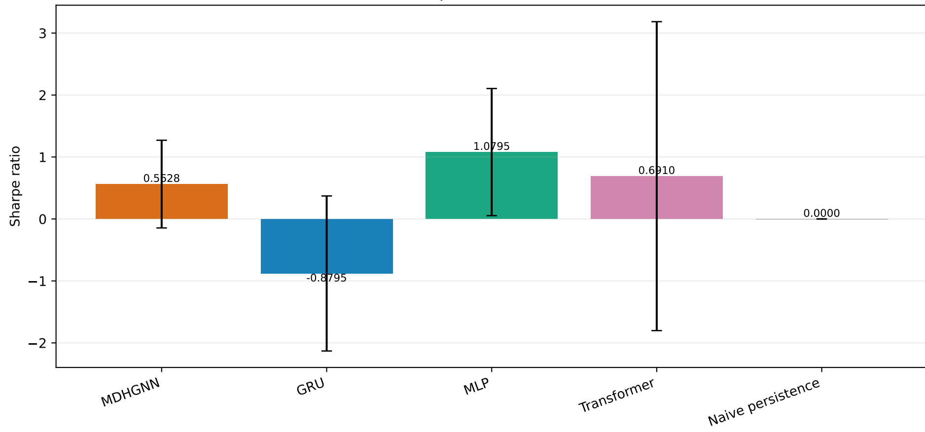
Model comparison on test set, h=2
