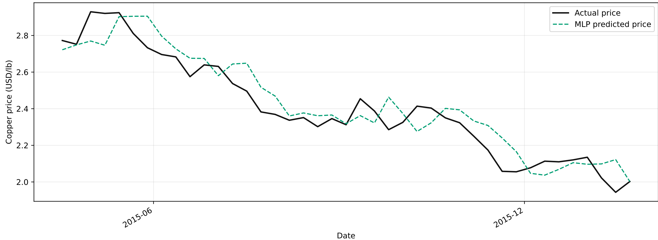
MLP prediction vs actual, h=2 Test period: 2015-04-17 to 2016-01-22
