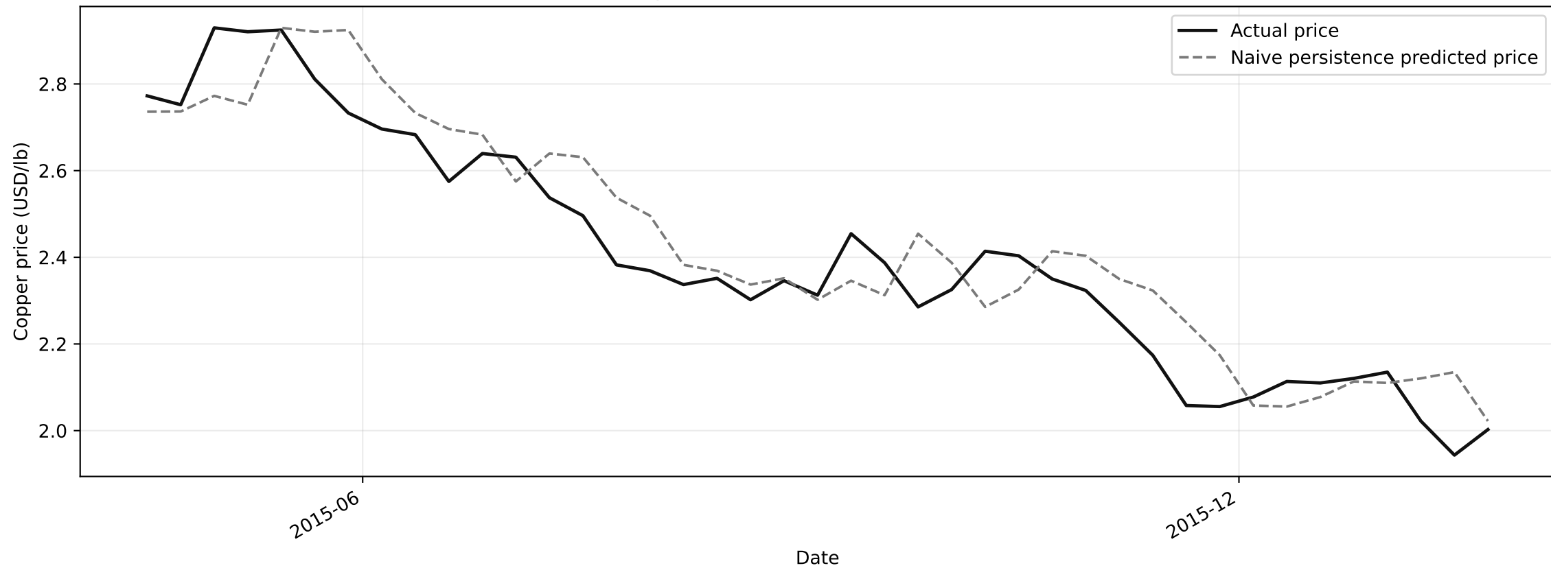
Naive persistence prediction vs actual, h=2 Test period: 2015-04-17 to 2016-01-22
