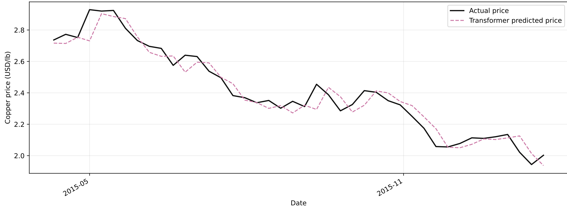
Transformer prediction vs actual, h=1 Test period: 2015-04-10 to 2016-01-22
