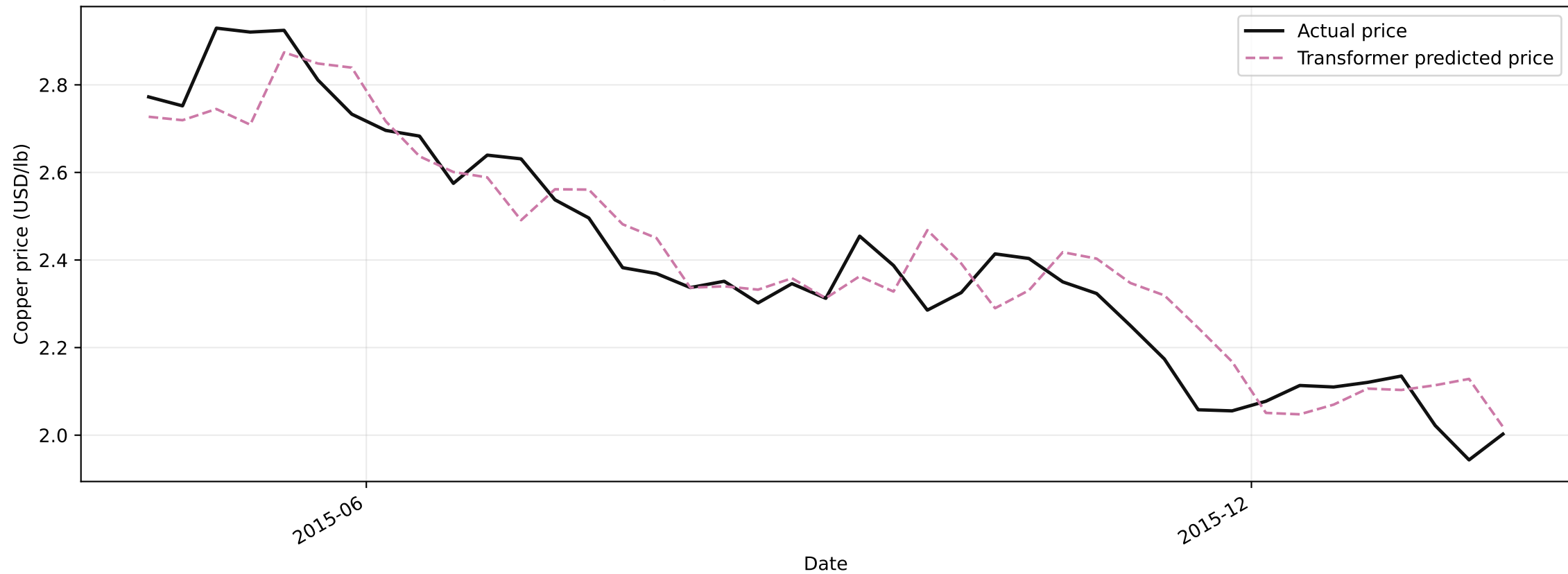
Transformer prediction vs actual, h=2 Test period: 2015-04-17 to 2016-01-22
