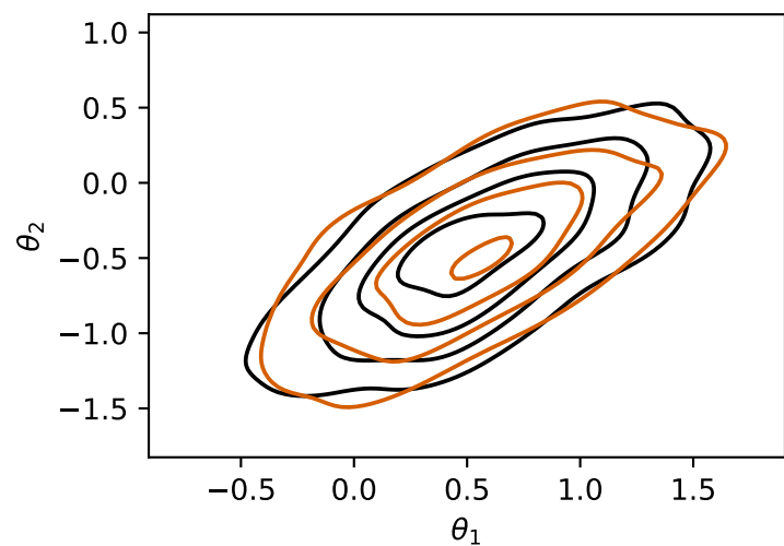
F-NPSE Langevin
