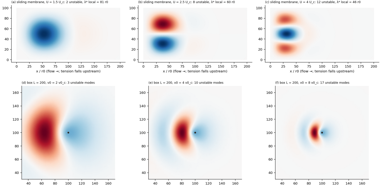
Figure 42: Plate-model modes well above onset and in sliding-membrane examples. Increasing compression permits multiple lobes and wrinkle trains; these modes do not establish a stable nonlinear pattern around a single protein.
