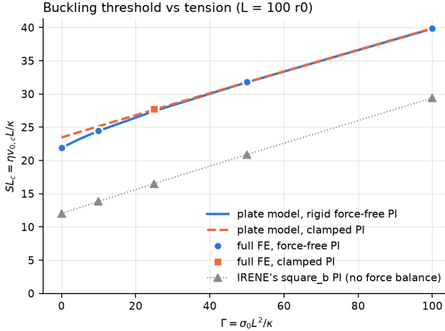
Figure 40: Critical drive with physical protein conditions. The rigid force-free and clamped formulations agree with their plate reductions. The lower grey curve uses the original free-rim condition without a vertical force equation and is retained only as a diagnostic. All thresholds refer to L = 100r_0 .
