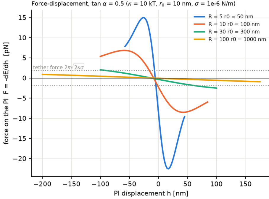
Figure 30: Mesh-converged force on the protein for \tan \alpha = 0.5 , plotted with the force convention F_m = -dE_*/dh . Upward holding-force maxima therefore appear as negative extrema. The dotted line denotes the magnitude of the long-tube force. Large rings have not reached their force extrema within this figure's displacement window.
