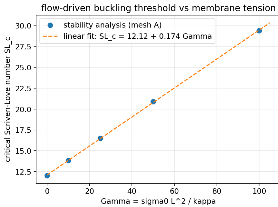
Figure 33: Superseded original-rim calculation. Its approximate linear threshold-versus-tension fit belongs to the implementation without vertical protein force balance and must not be used for the corrected physical model.
