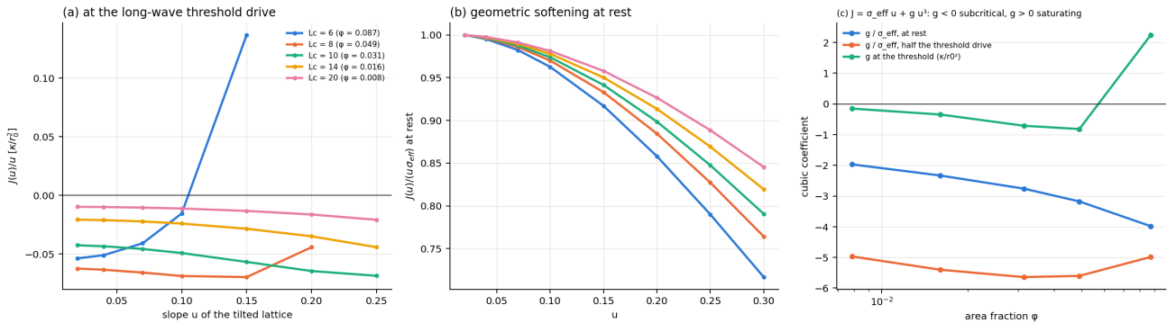
Figure 62: Nonlinear tilted-cell stress and geometric softening. Frozen flat-state flow is used; the small-slope cubic changes sign between intermediate and dense arrays, while the driven linear coefficient differs modestly from the dynamic Bloch value.
