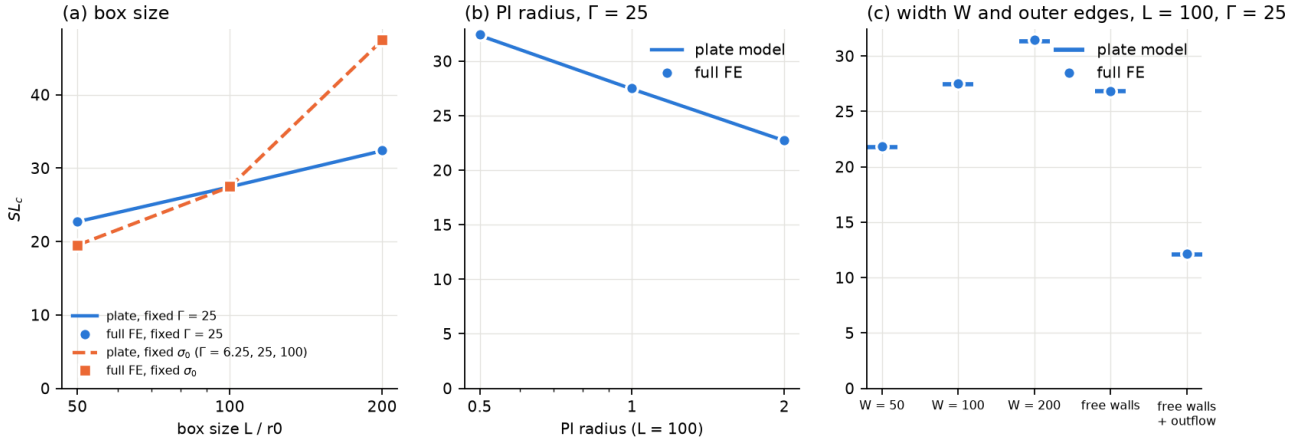
Figure 43: Corrected physical thresholds versus domain length, protein radius, width, and outer-height constraints. Fixed-tension and fixed- \Gamma size sweeps are different experiments.
