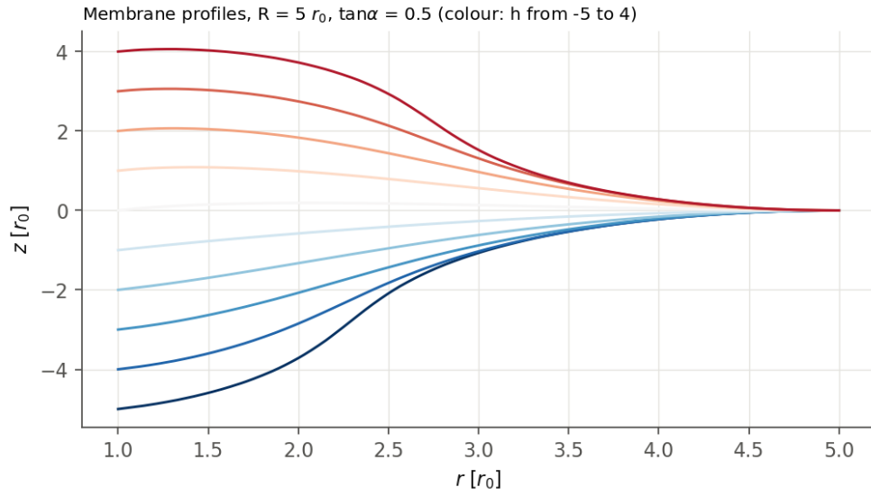
Figure 28: Strongly confined ring profiles at outer radius R = 5r_0 . Large end slopes limit a height representation and distinguish the confined neck from a freely developed wide tube.
