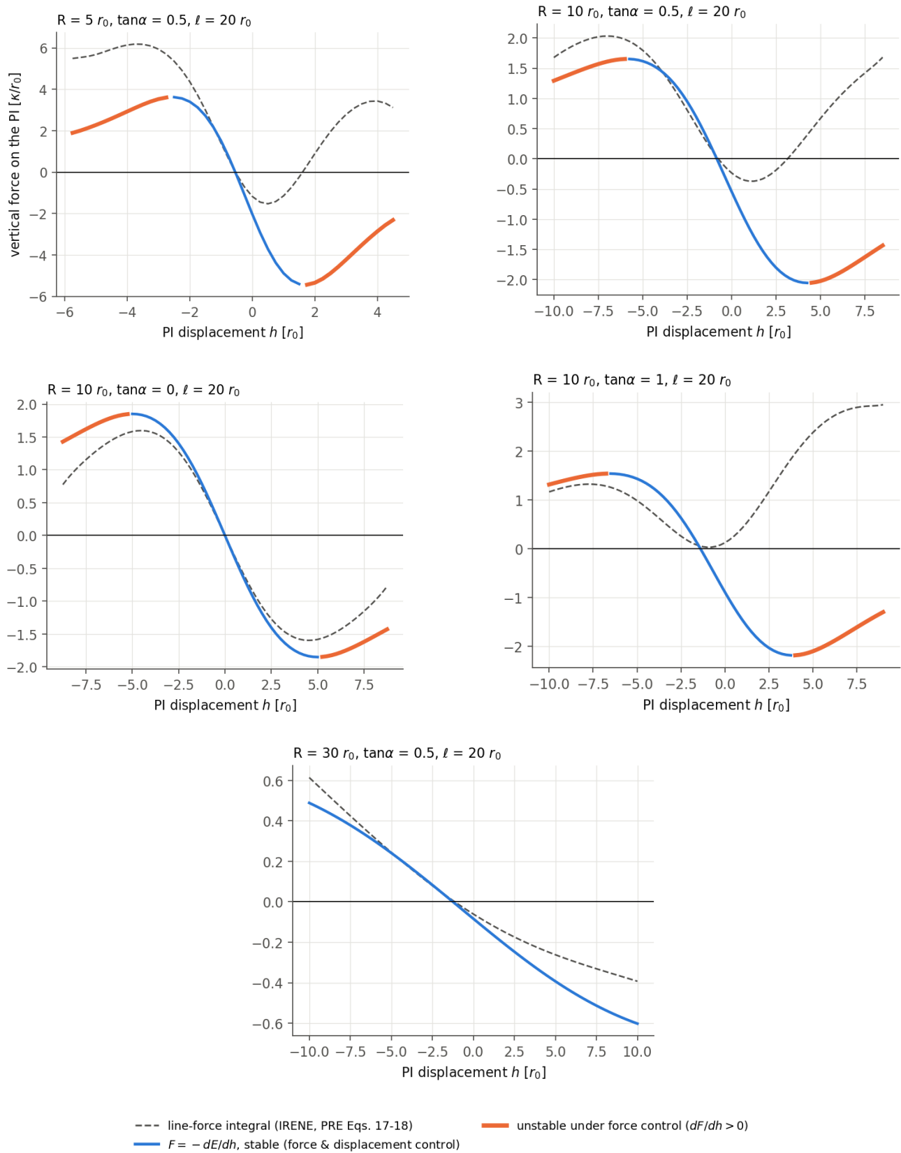
Figure 22: Ring forces and fixed-height eigenvalues for several radii. Dashed original line-force curves are retained as diagnostics; extrema and force-control conclusions use virtual work.
