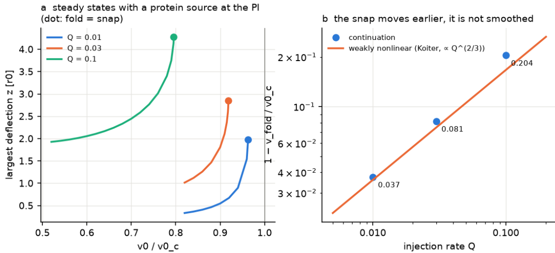
Figure 60: Source-induced folds and the Koiter prediction. Recruitment is an imperfection that advances rather than removes the snap. The largest-source case is outside the smallest-amplitude cubic regime.
