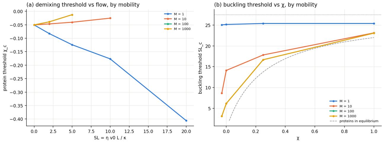
Figure 58: Mobility dependence of demixing and buckling with absorbing outflow. Slow diffusion suppresses global demixing and changes the buckling threshold modestly. Fast diffusion permits curvature relaxation and merges the two instability sectors. Intermediate mobility produces travelling modes. These sweeps use the rigid force-free flat-state condition; the separate codimension-two analysis uses a clamped protein.
