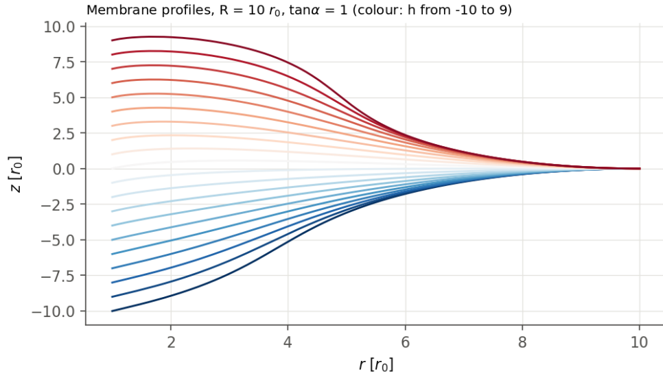
Figure 27: Ring profiles at outer radius R = 10r_0 and unit contact slope. The imposed slope biases the spontaneous height and the two force-control barriers.
