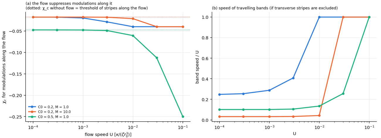
Figure 55: Uniform-plane curvature–protein dispersion under relative drift. Transverse wavevectors remain least affected, giving stripes parallel to the flow; travelling longitudinal bands require suppressing those transverse modes.
