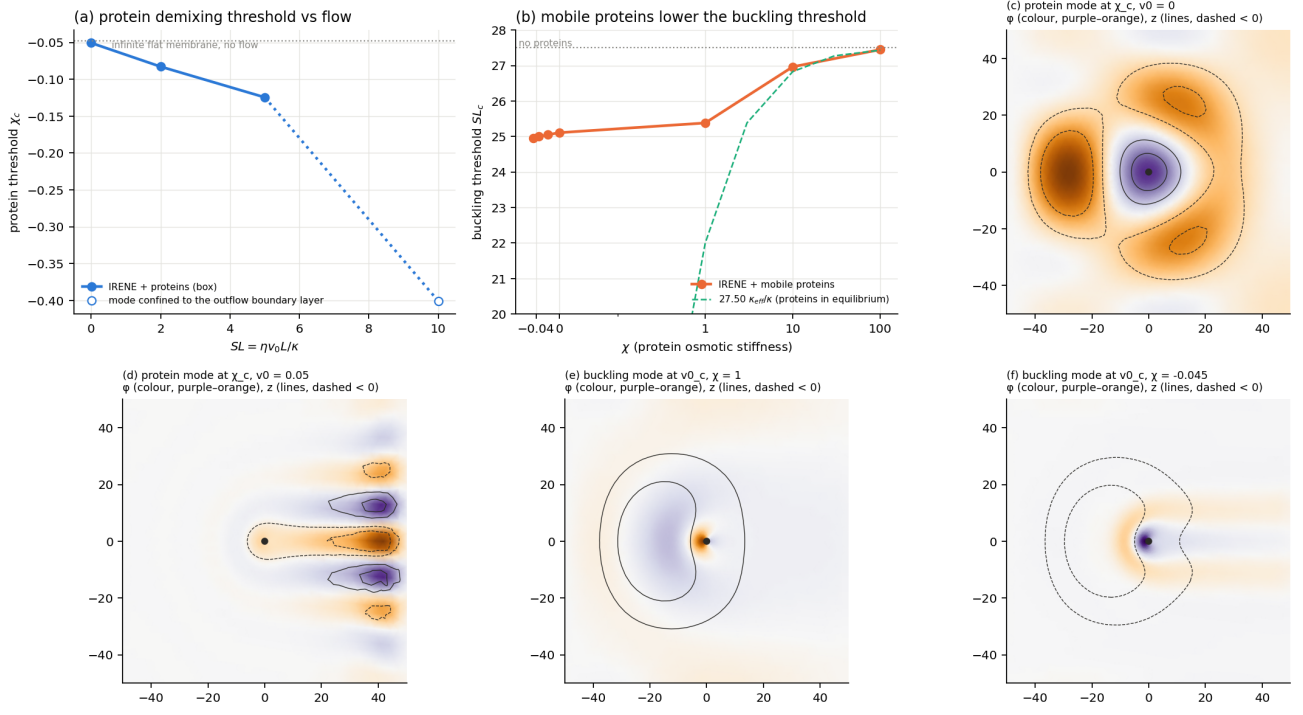
Figure 57: Earlier mobile-protein thresholds with no-flux outflow. The high-flow demixing mode is an outflow-layer artifact. The final absorbing-outflow mobility study replaces those high-flow thresholds.
