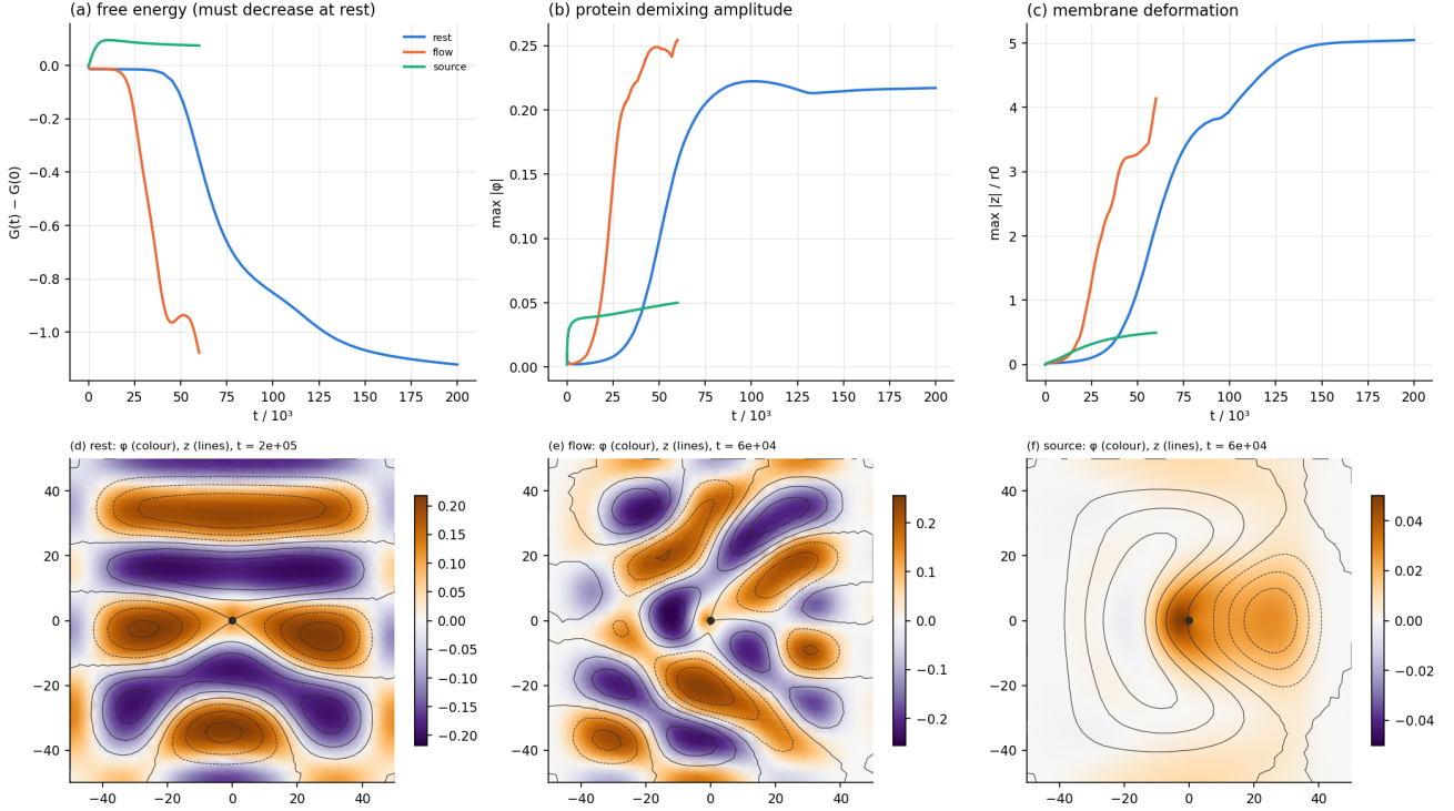
Figure 56: Consistent nonlinear mobile-protein dynamics: no-flow energy relaxation, amplitude saturation, flow-elongated domains, and a source-driven plume. Open reservoirs/sinks mean global protein conservation must include boundary exchange.
