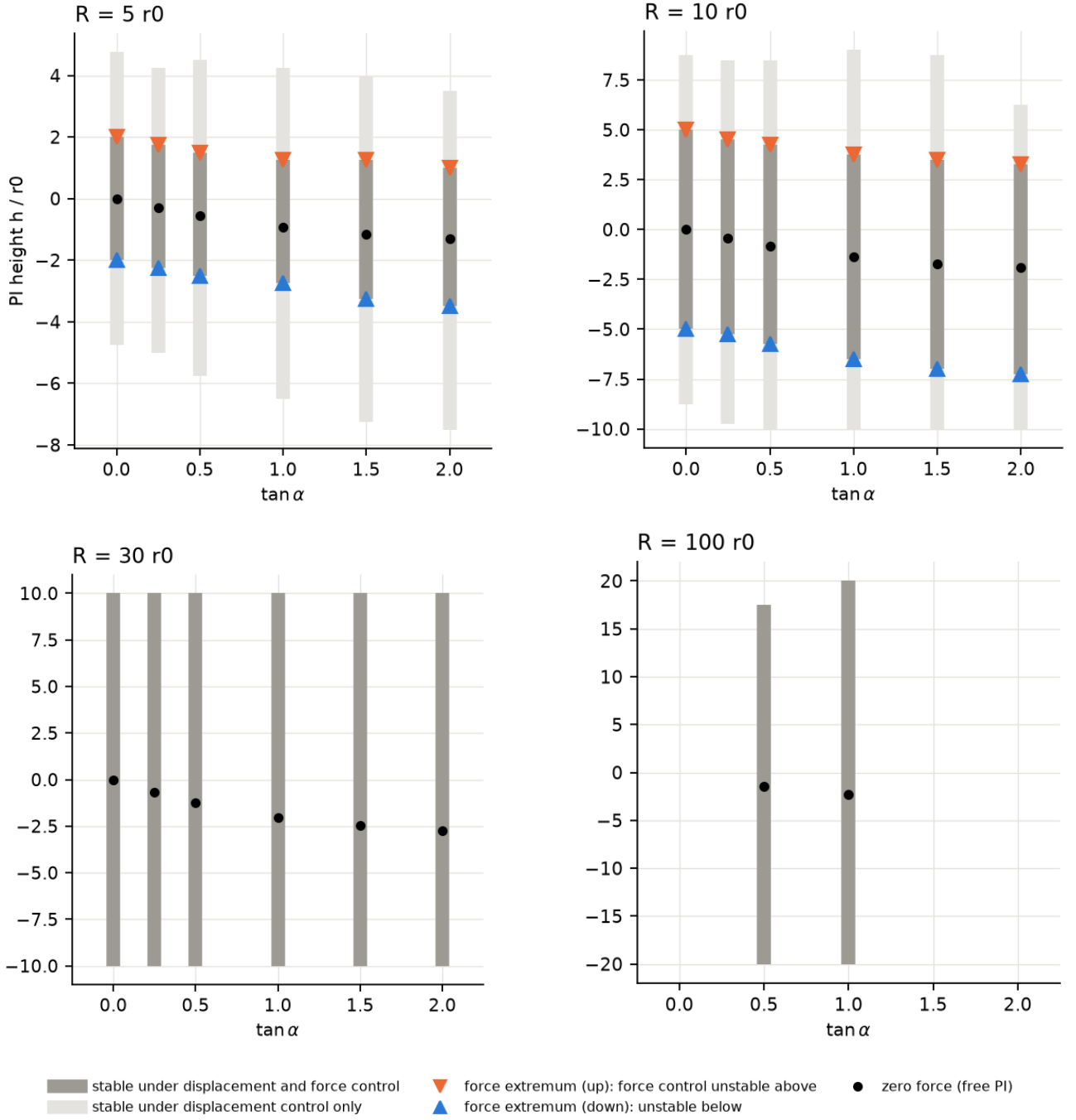
Figure 24: Height/contact-slope ring stability diagram over the computed windows. The force-control boundaries are virtual-work force extrema; height-controlled branches remain stable. Grey endpoints indicate limits of the sampled branch.
