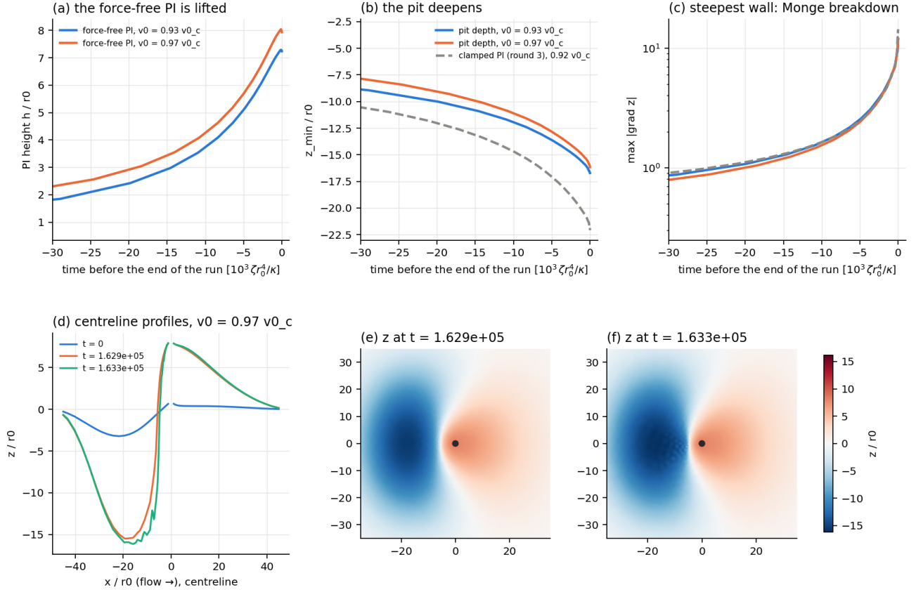
Figure 50: Force-free protein lift during upstream collapse. The protein rises onto a downstream crest and the wall steepens; cutoff-force consistency deteriorates at the last slopes.
