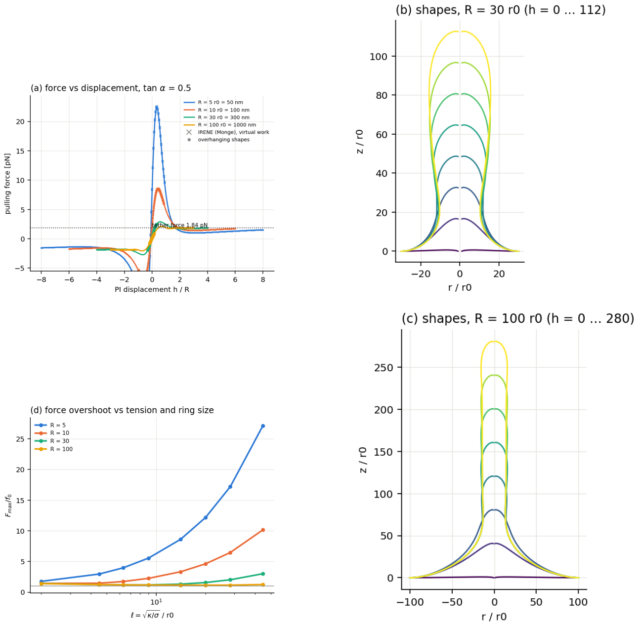
Figure 31: No-flow axisymmetric arclength continuation. Large rings develop tubes tending to the tether-force plateau; small rings constrain a neck and show a large force overshoot. This axisymmetric equilibrium calculation does not resolve the asymmetric flow-driven tube evolution.
