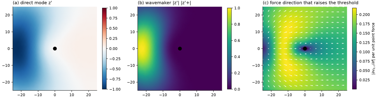
Figure 44: Normal direct/adjoint shape, wavemaker, and tangential-force direction that increases the reference threshold. The strong response is located upstream of the inclusion.
