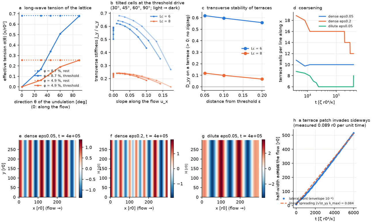
Figure 65: Two-dimensional lattice reduction. Long-wave stiffness is softened along the flow but remains positive transversely. Straight terrace ridges run across the flow. Positive transverse terrace stiffness excludes a zigzag in the tested dense and intermediate-density cases. A localized patch spreads laterally at a speed close to the linear pulled-front prediction.
