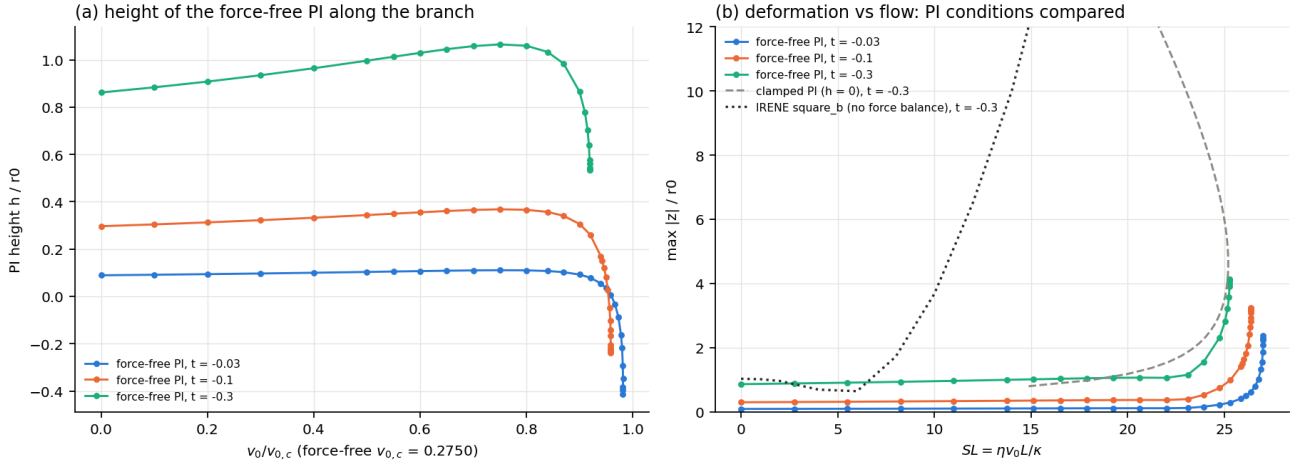
Figure 48: Nonlinear force-free branches for nonzero contact slopes, contrasted with clamped and original-rim conditions. The corrected free protein stays near its rest deformation before an imperfection-sensitive fold.
