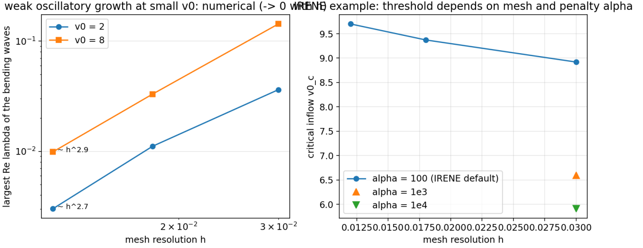
Figure 39: Slip-penalty example: weak oscillatory growth shrinks with mesh size, while the apparent threshold depends strongly on penalty strength. These results diagnose numerical and boundary-condition sensitivity and are excluded from the quantitative buckling predictions.
