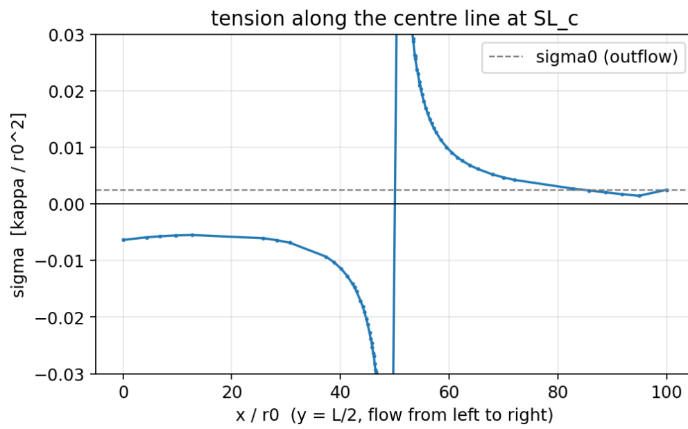
Figure 35: Original-rim flat base-flow tension along the centreline. The upstream tension decrease is mechanistic evidence; the onset value attached to this figure is superseded by the physical protein condition.
