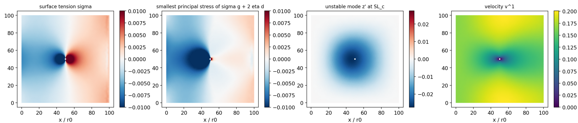
Figure 34: Superseded original-rim stress and eigenmode fields. They reveal upstream compression but place the mode nearer the protein than the corrected force-balanced problem.
