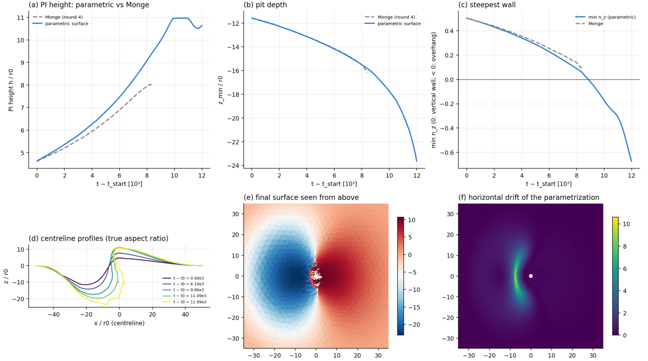
Figure 51: Continuation of the force-free post-snap state on a parametric surface, compared with the Monge calculation. True-aspect-ratio centreline profiles show the wall turning over beneath the elevated protein. The final large-deformation state is limited by mesh distortion; it is not a completed tube.
