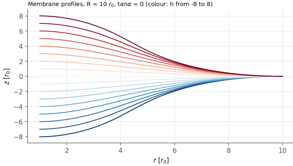
Figure 25: Symmetric zero-contact-slope ring profiles at outer radius R = 10r_0 . Upward and downward branches are related by reflection in the reference plane.
