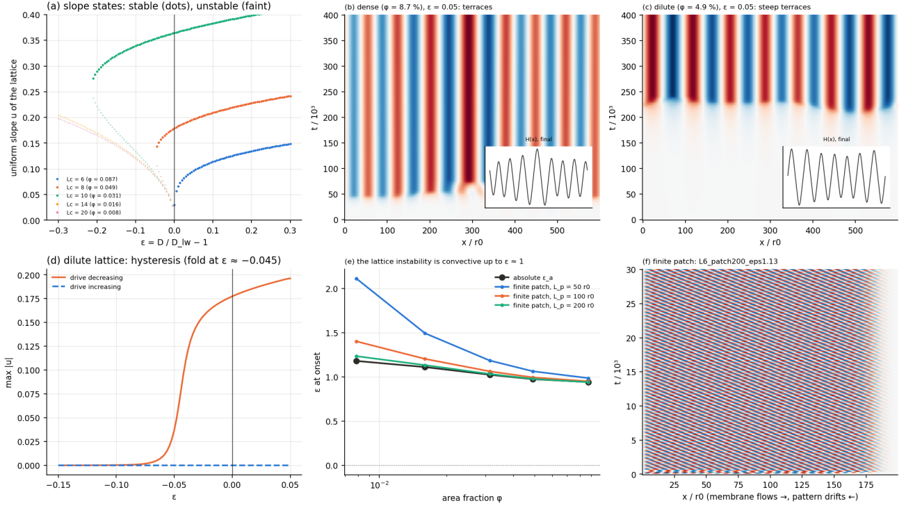
Figure 64: One-dimensional homogenized lattice dynamics: continuous or hysteretic slope states, coarsening terraces, and finite-patch drift. The absolute-threshold estimate uses a long-wave model near the edge of its spatial validity.
