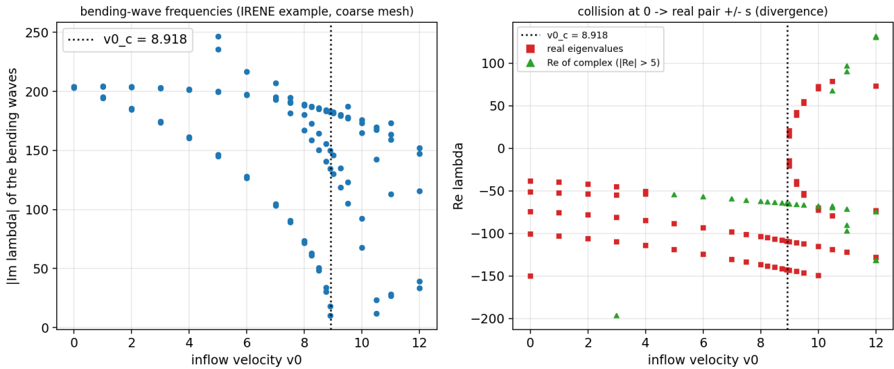
Figure 38: Inertial bending-wave collision in the slip-inclusion example. This is an illustrative high-inertia mechanism, not the overdamped lipid-membrane threshold.
