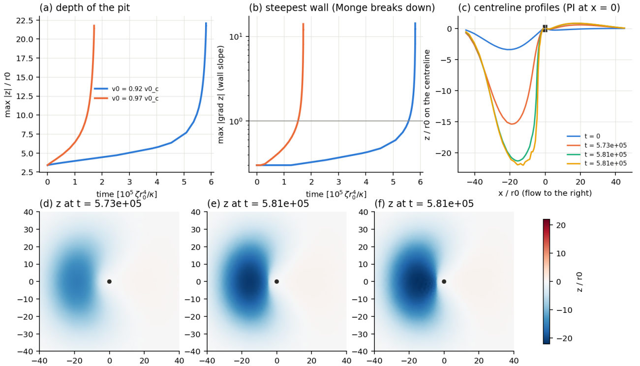
Figure 49: Clamped-protein time stepping after the fold: bottleneck, deepening upstream pit, and rapid slope growth. The final steep shapes are at the Monge limit, not resolved steady attractors.
