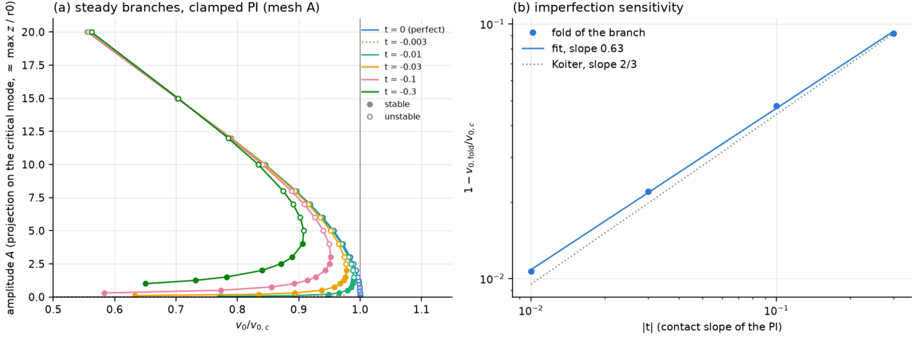
Figure 46: Corrected clamped-protein continuation. The perfect branch is subcritical and a nonzero contact slope produces a fold; the fitted imperfection exponent is close to two thirds. The residual projection in Section 11 supplies an independently computed prefactor.
