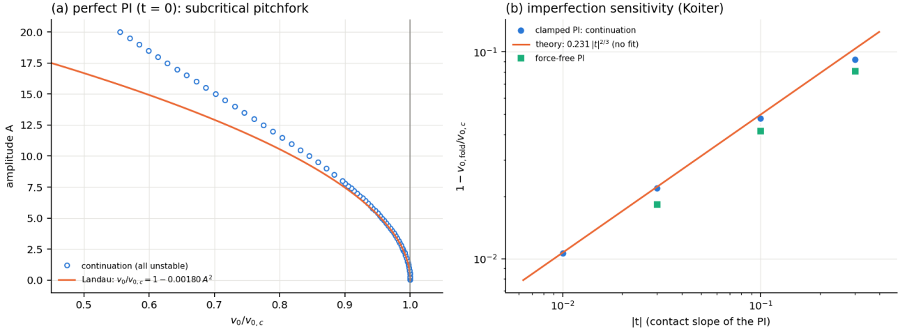
Figure 47: Weakly nonlinear predictions against full continuation. The perfect branch bends backward, establishing subcritical buckling. The imperfection law includes a coefficient computed from the equations. Clamped and force-free fold data are distinct; the displayed clamped theory is not a fitted force-free formula.
