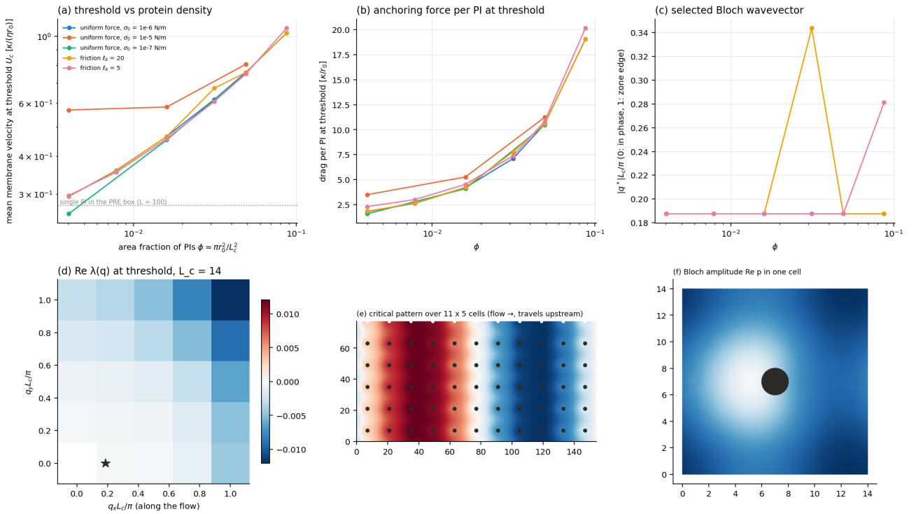
Figure 61: Periodic array spectra and patterns. Early finite-wavevector scans are interpreted with the dedicated later long-wave coefficients: a neutral uniform translation exists at zero wavevector, and the longitudinal stiffness controls onset.
