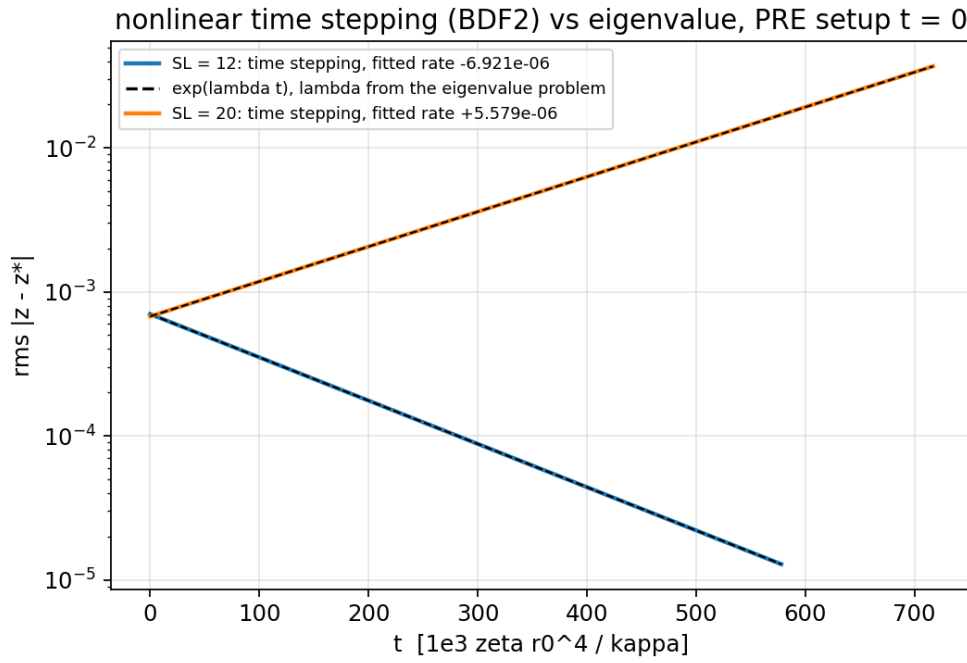
Figure 37: BDF2 versus eigenvalue growth and decay for the original-rim implementation. This checks that the numerical linearization predicts that implementation's dynamics, not that its rim condition is physically force-free.
