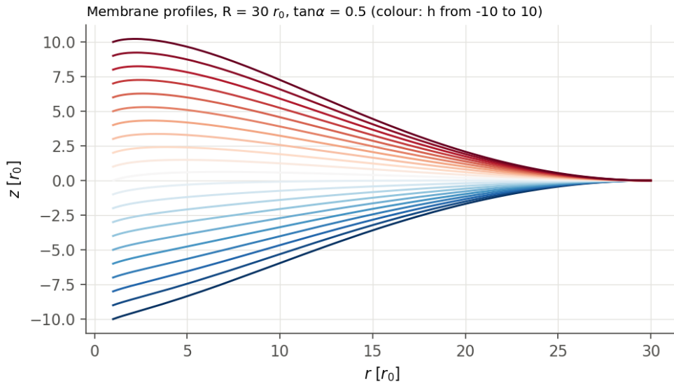
Figure 29: Profiles for outer radius R = 30r_0 and contact slope s = 0.5 . The displayed Monge window does not reach the long-tube force plateau.
