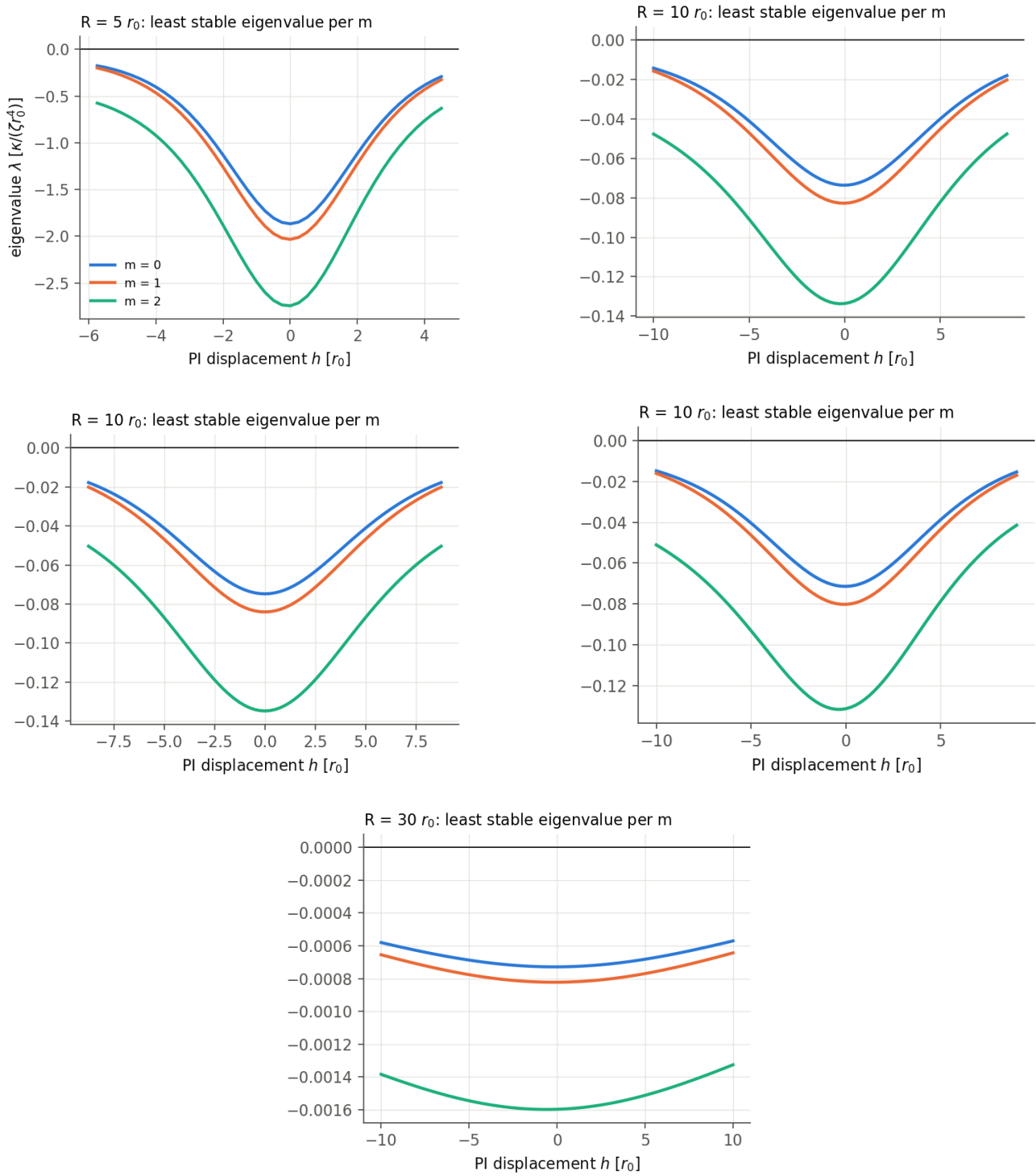
Figure 21: Ring relaxation spectra versus protein height, resolved by azimuthal number. No growing fixed-height mode is found in these sampled branches; spectra soften as the neck becomes steep.
