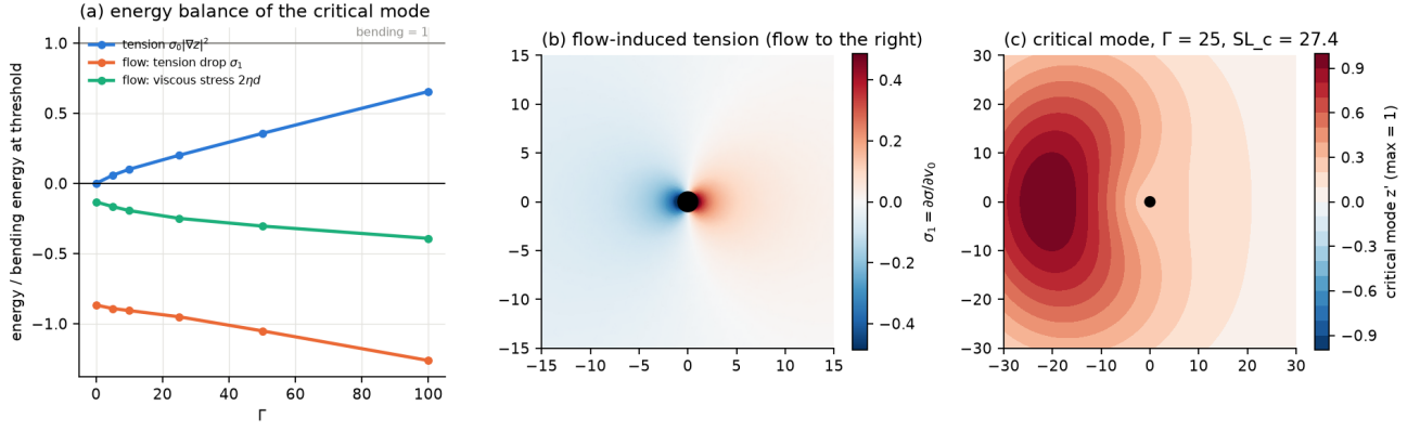
Figure 41: Energy decomposition, flow-induced tension, and the critical mode of the corrected flat-state problem. The tension falls upstream of the no-slip obstacle, and the critical deflection lies upstream rather than being centred on the protein. The negative flow contribution balances bending and the imposed tension.
