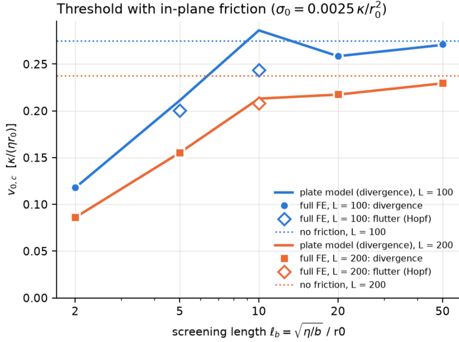
Figure 52: Early friction comparison showing divergence thresholds and full-equation flutter crossings. The real plate threshold curve alone is not the first onset when a complex pair crosses earlier; the subsequent divergence–flutter map resolves this.
