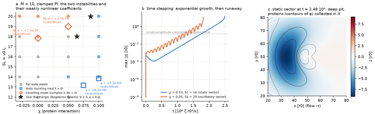
Figure 59: Clamped-protein, intermediate-mobility eigenvalue sectors and nonlinear runaway. The nearly vanishing eigenvalues motivate a degenerate Bogdanov–Takens-type interpretation; an exact double-zero location and quintic unfolding remain unresolved.
