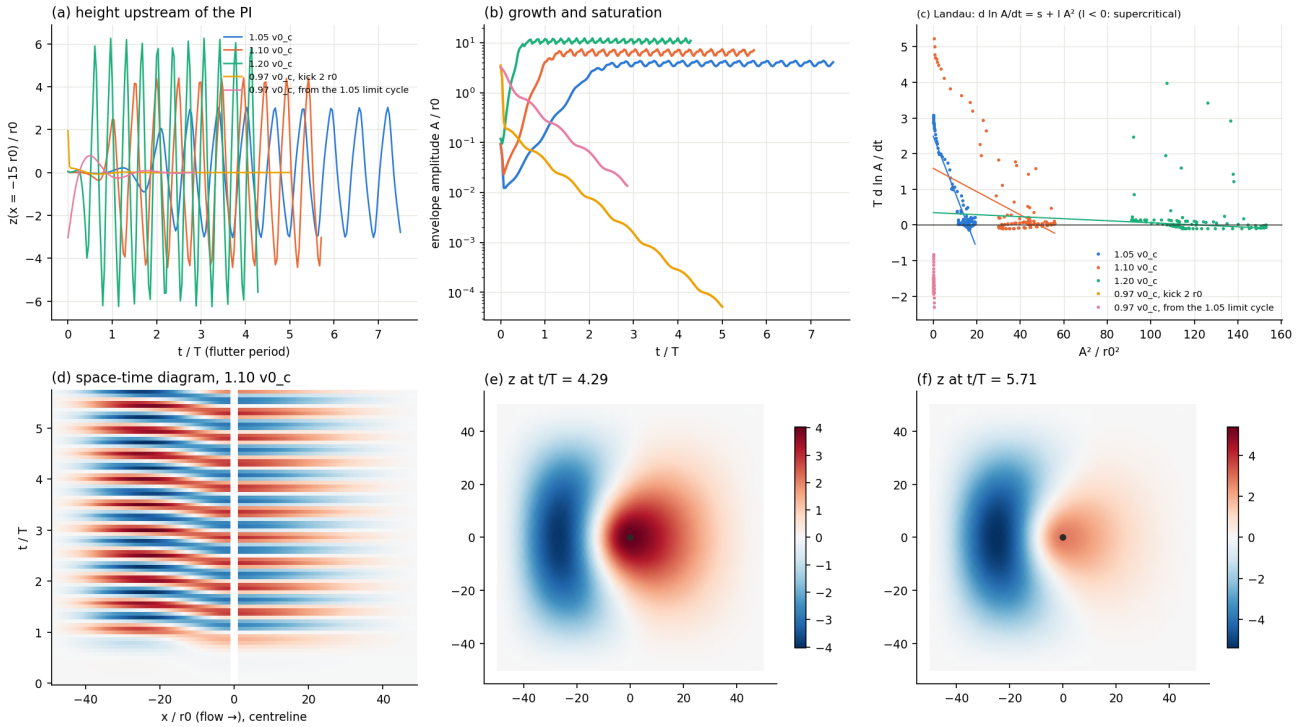
Figure 54: Nonlinear flutter at \ell_b = 7r_0 , \Gamma = 25 , and a rigid force-free protein. Growth saturates above onset, and the space-time bands reveal upstream propagation. Bounded oscillations and decay after a below-threshold restart establish saturation in the tested trajectories; a near-onset cubic coefficient and full periodic-orbit stability remain to be determined.
