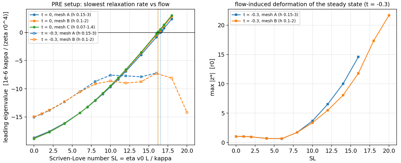
Figure 32: Superseded original-rim flow spectra and large imperfect deformation. The threshold near SL = 16 is a diagnostic of the original boundary-value problem; corrected thresholds are near SL = 27.45 in the reference geometry.
