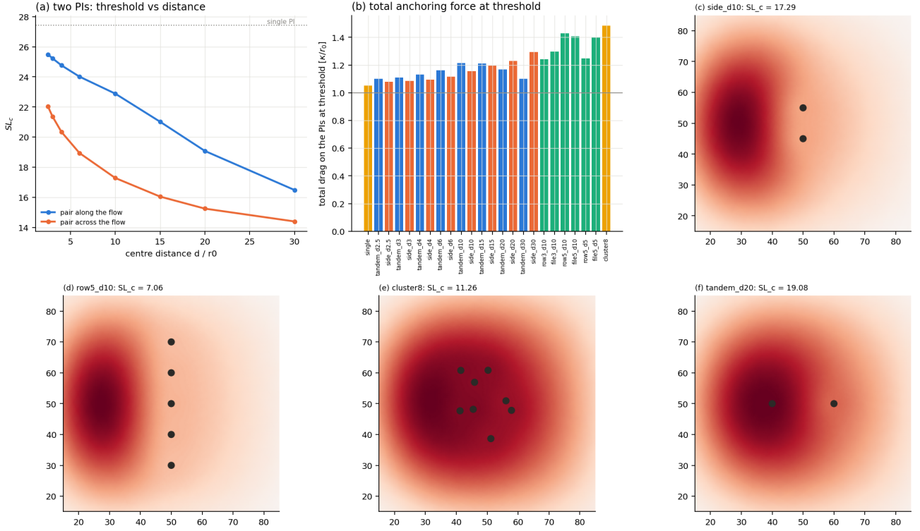
Figure 45: Finite protein groups: arrangement-dependent thresholds, total anchoring drag at onset, and collective critical shapes. The force plotted in panel (b) is the sum over all inclusions in the finite patch. The clustering of this quantity is much tighter than that of the critical drive.
