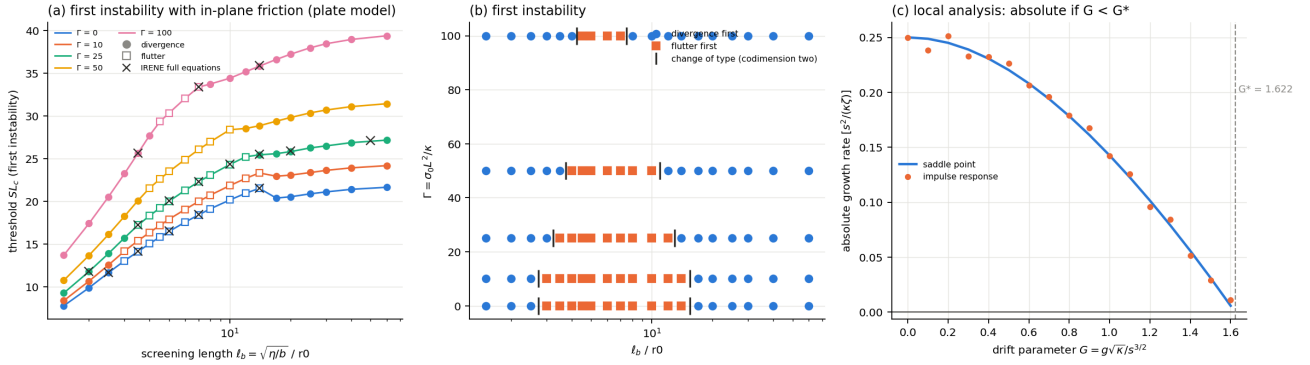
Figure 53: Divergence/flutter onset map versus screening length and tension, with full-equation checks. The local absolute-instability panel is a guide to the global wave source; near onset the local wavelength is comparable to the compressed region.
