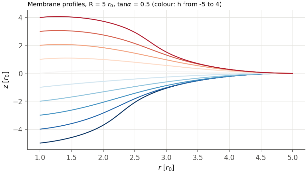
Figure 30: Strongly confined ring profiles at outer radius R = 5r_0 . Large end slopes limit a height representation and distinguish the confined neck from a freely developed wide tube.
