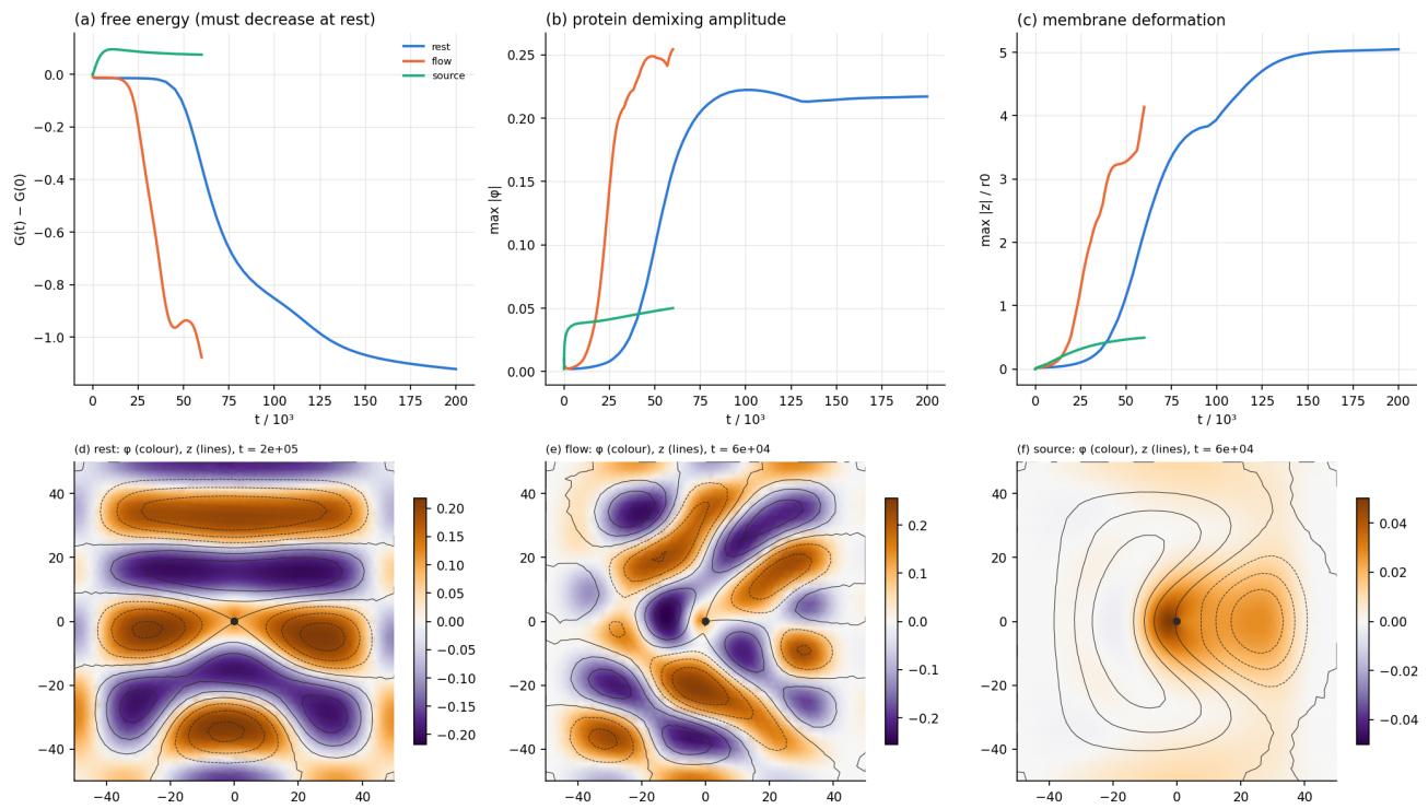
Figure 69: Consistent nonlinear mobile-protein dynamics: no-flow energy relaxation, amplitude saturation, flow-elongated domains, and a source-driven plume. Open reservoirs/sinks mean global protein conservation must include boundary exchange.
