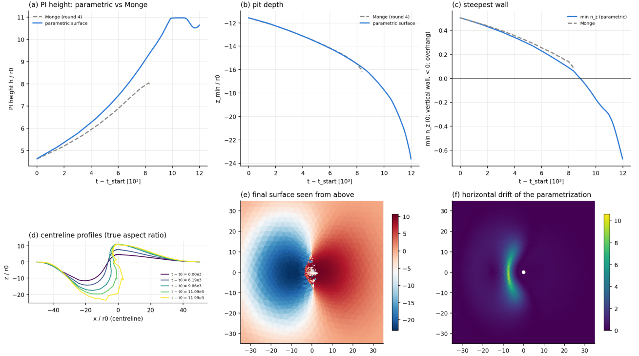
Figure 61: Continuation of the force-free post-snap state on a parametric surface, compared with the Monge calculation. True-aspect-ratio centreline profiles show the wall turning over beneath the elevated protein. The final large-deformation state is limited by mesh distortion; it is not a completed tube.
