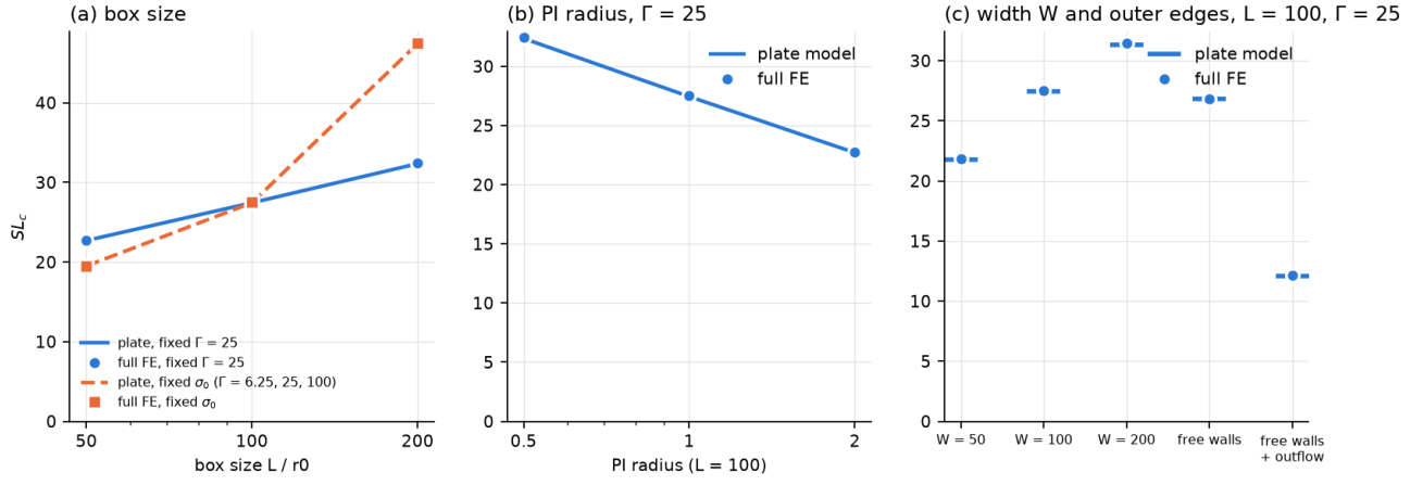
Figure 51: Corrected physical thresholds versus domain length, protein radius, width, and outer-height constraints. Fixed-tension and fixed-Gamma size sweeps are different experiments.
