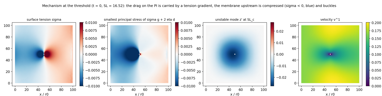
Figure 41: Superseded original-rim stress and eigenmode fields. They reveal upstream compression but place the mode nearer the protein than the corrected force-balanced problem.
