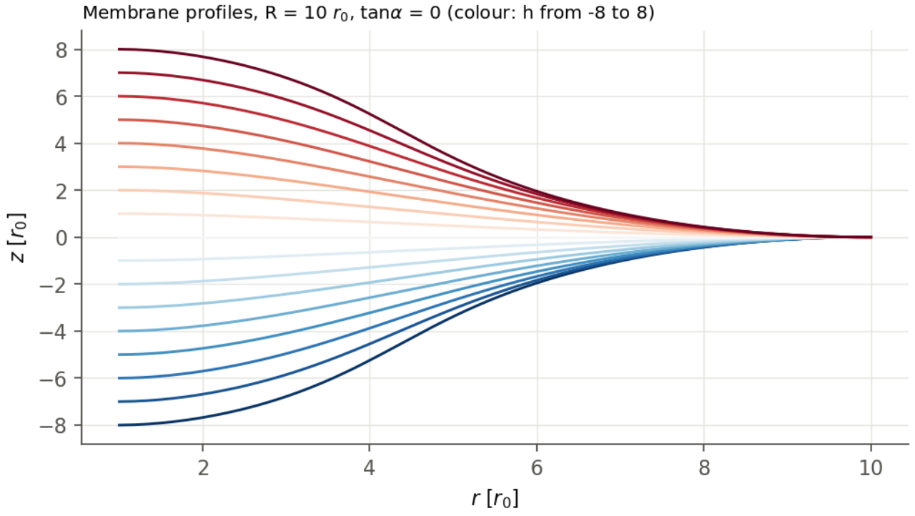
Figure 30: Symmetric zero-contact-slope ring profiles at outer radius ten. Upward and downward branches are related by reflection in the reference plane.
