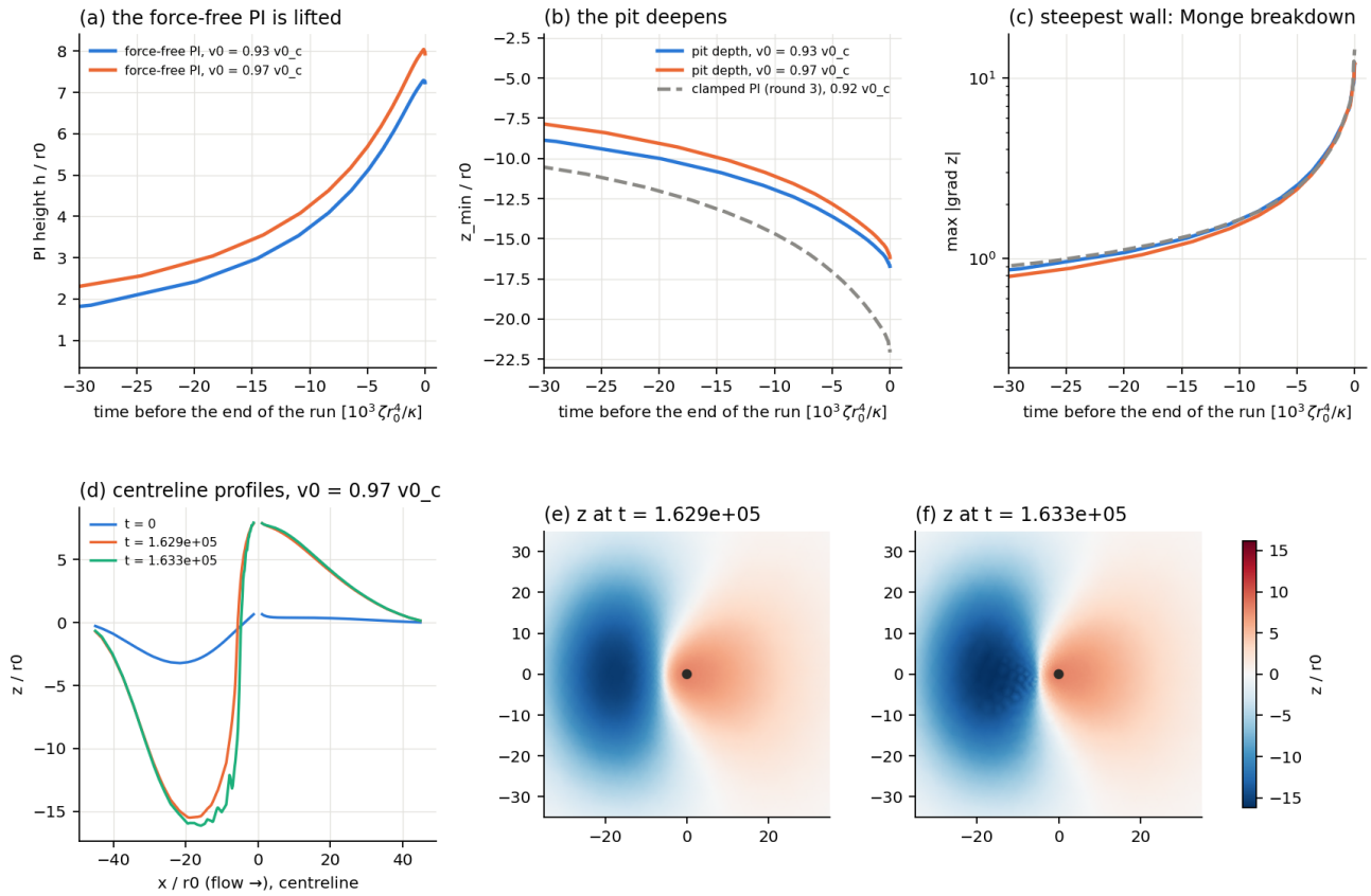
Figure 50: Force-free protein lift during upstream collapse. The protein rises onto a downstream crest and the wall steepens; cutoff-force consistency deteriorates at the last slopes.
