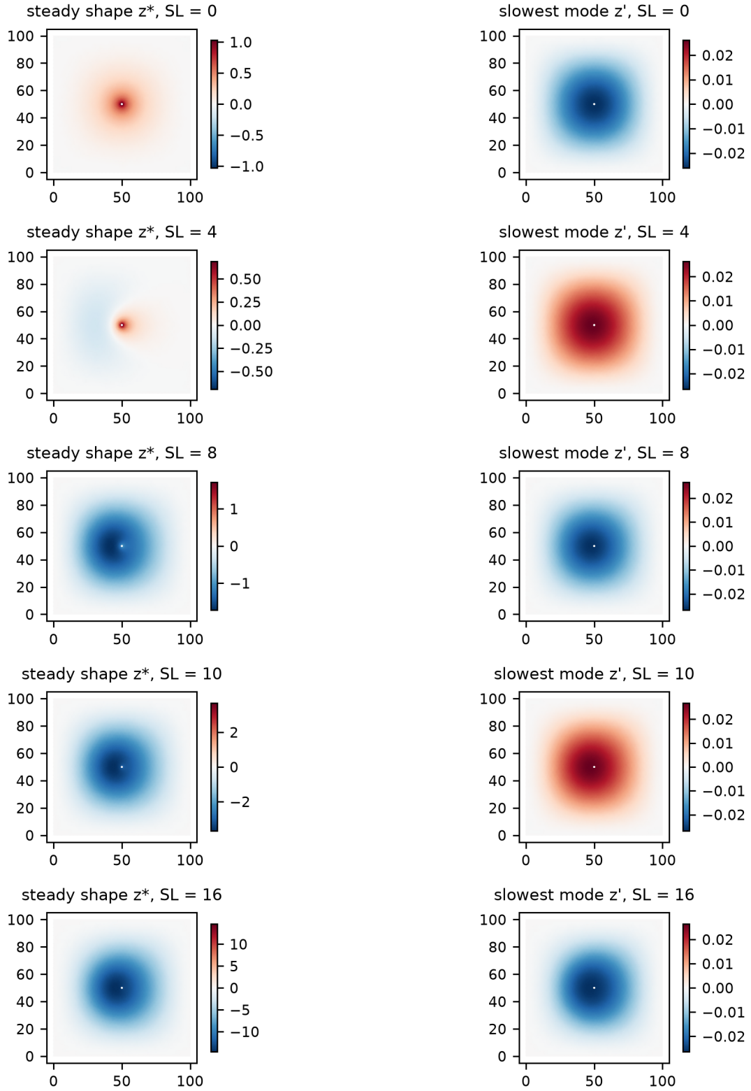
Figure 36: Superseded original-rim shapes and leading modes at nonzero contact slope. Their large smooth deformation is not evidence for a smooth transition with a physically force-free protein.
