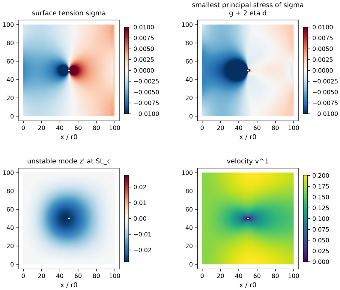
Figure 34: Superseded original-rim stress and eigenmode fields. They reveal upstream compression but place the mode nearer the protein than the corrected force-balanced problem.
