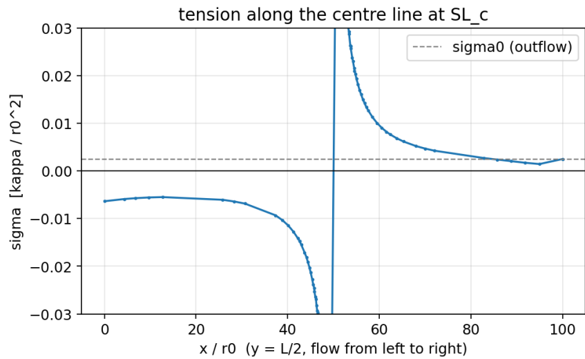
Figure 35: Original-rim flat base-flow tension along the centreline. The upstream tension decrease is mechanistic evidence; the onset value attached to this figure is superseded by the physical protein condition.
