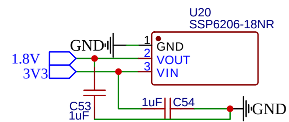
3.3v转1.8V电路
