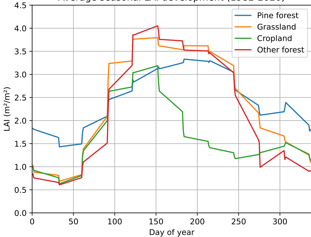
Average seasonal LAI development (1982-2020)
