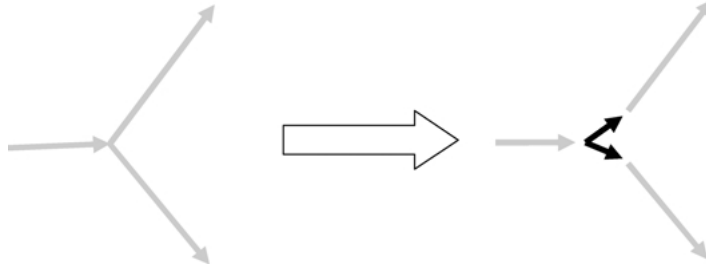
Figure 6. Node expansion.
