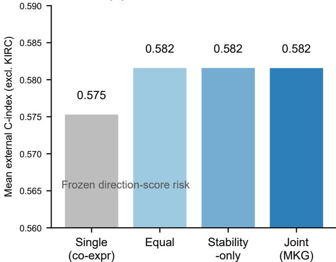
(A) Submission-lock ablation
