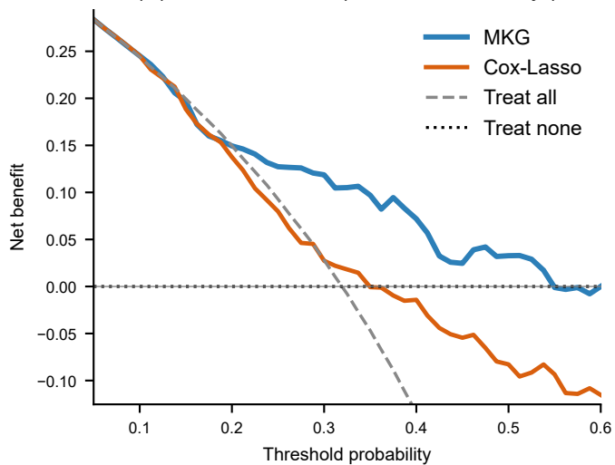
(B) Decision curve (LIHC external, 3-yr)
