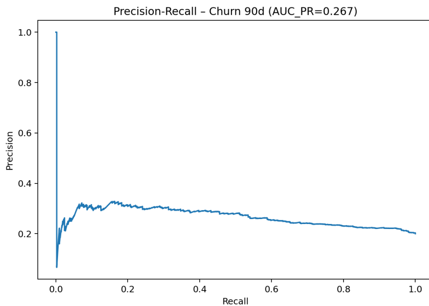
PR – churn
