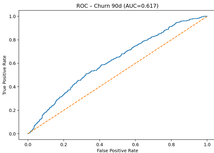
ROC – churn
