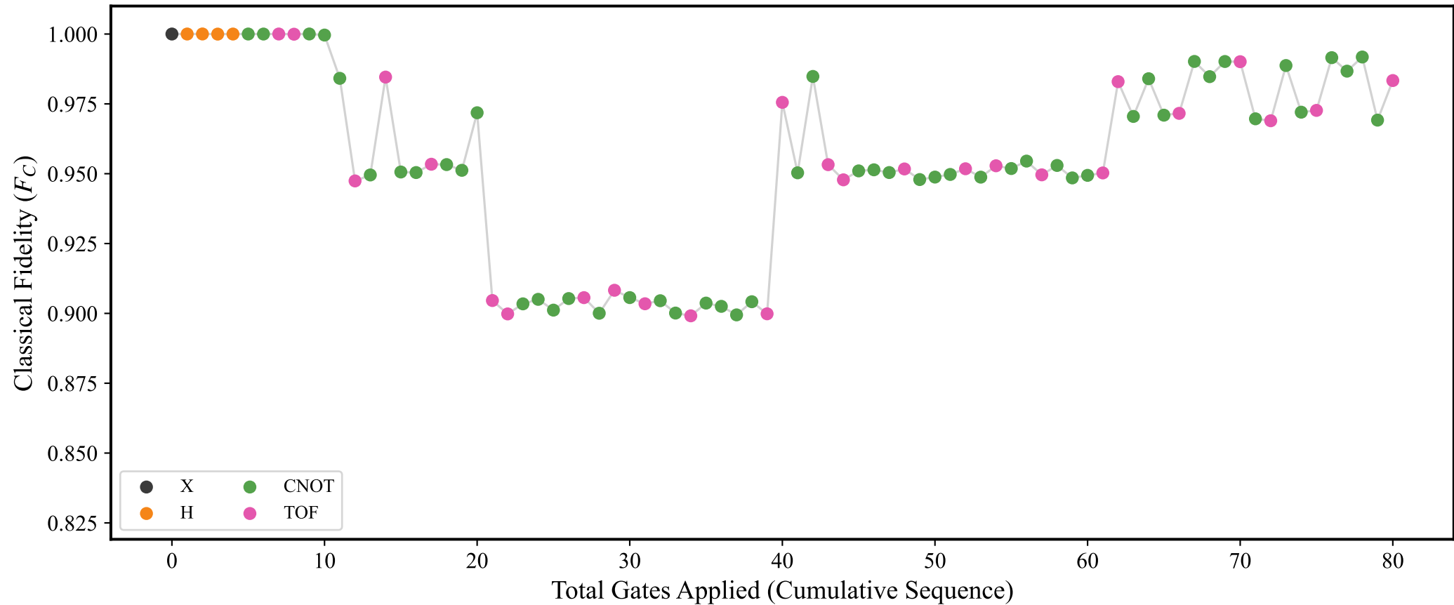
Modular Exponentiation for N=3 , a=2 (12-Qubit VBE Circuit)
