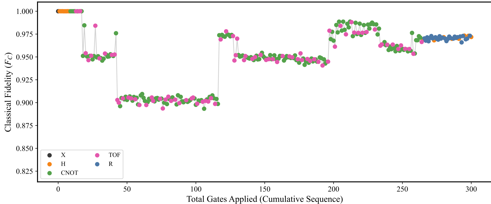
Shor's Algorithm for N=15 , a=4 (22-Qubit VBE Circuit)
